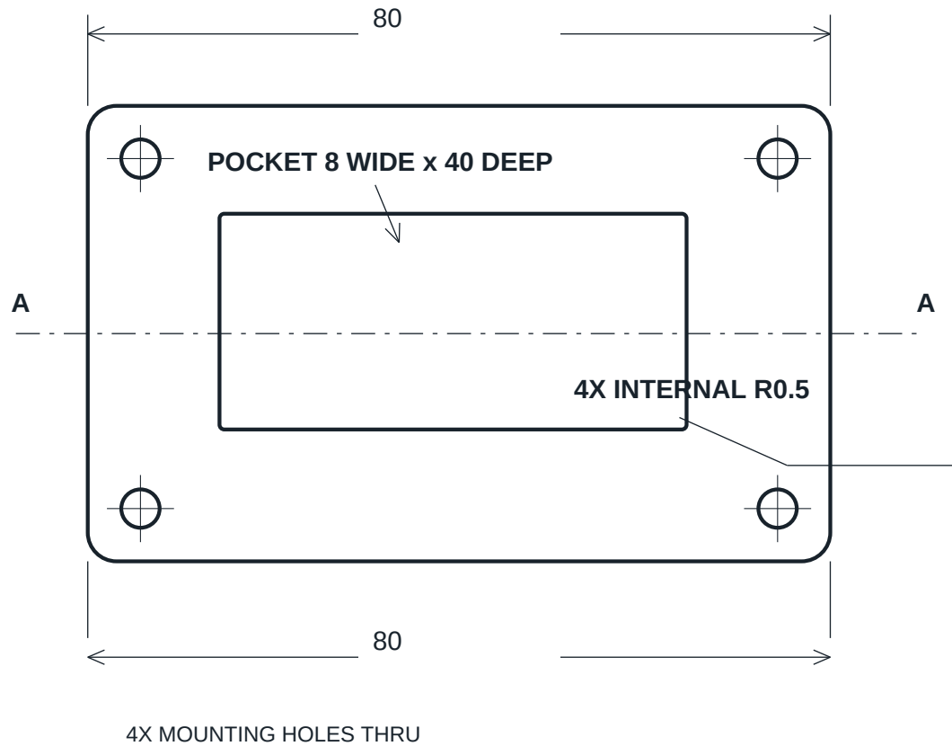
01 PLAN VIEW
