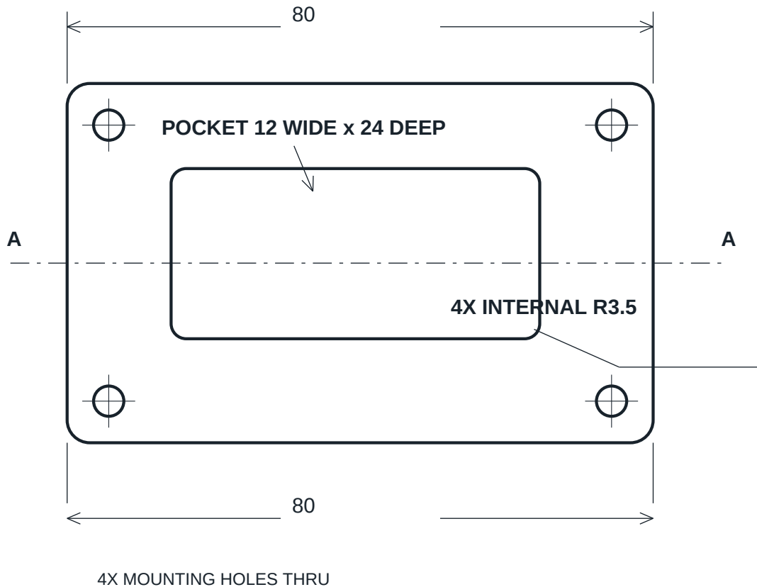
01 PLAN VIEW
