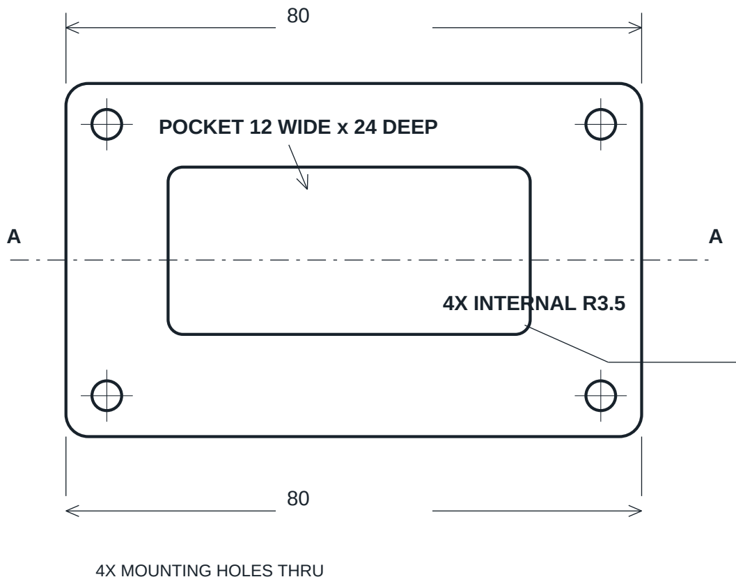
01 PLAN VIEW
