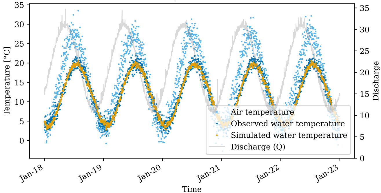
Calibration, RMSE=1.1215°C
