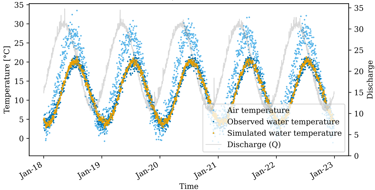
Calibration, RMSE=1.1506°C
