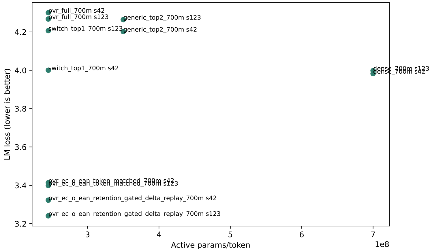
700M Active Params vs LM Loss
