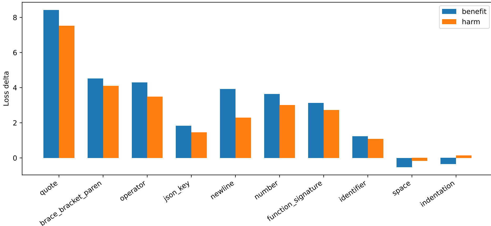
Expert Causality by Token Class
