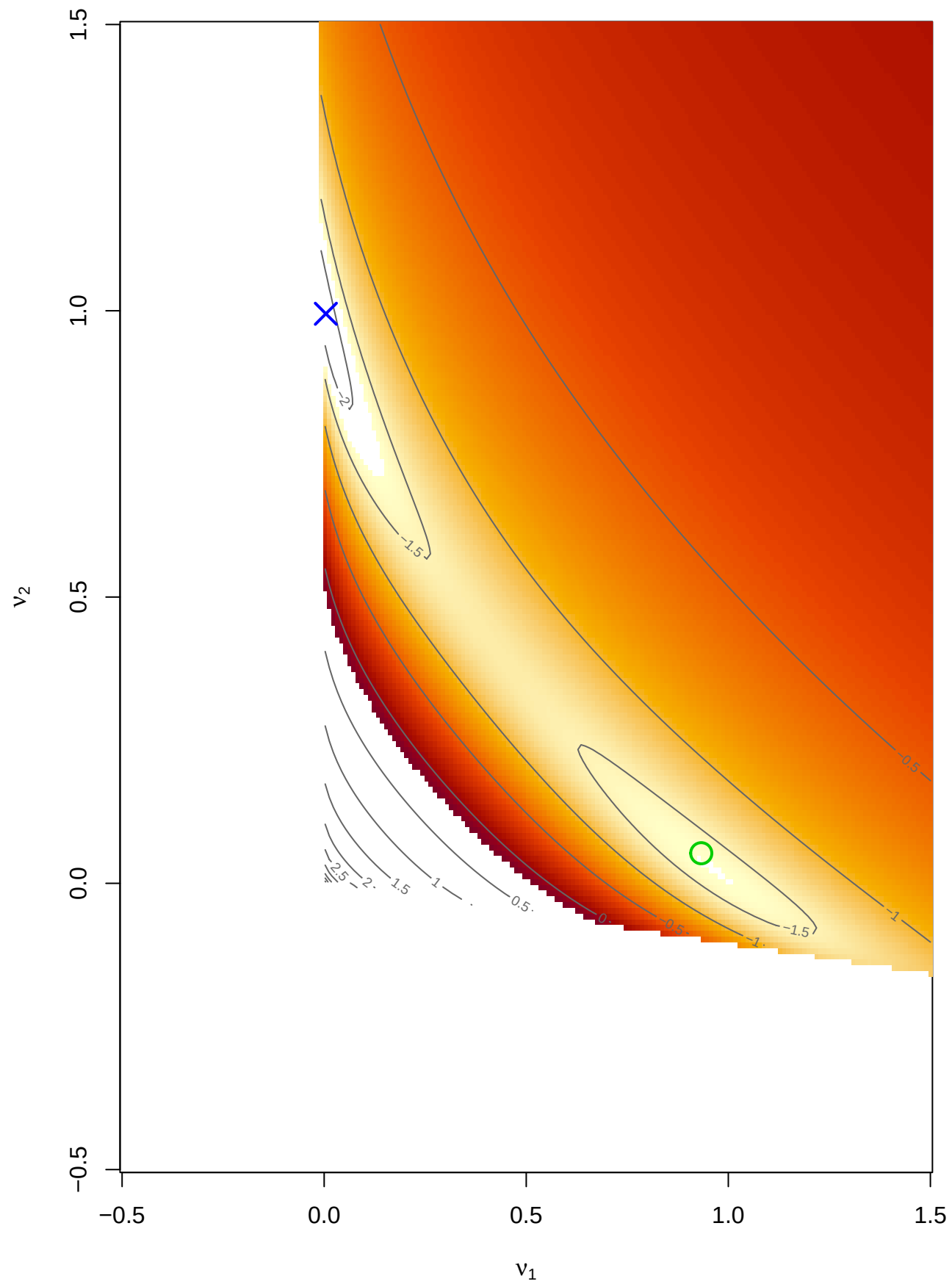
Rep 4: Fixed W=I , G'G (log10)
