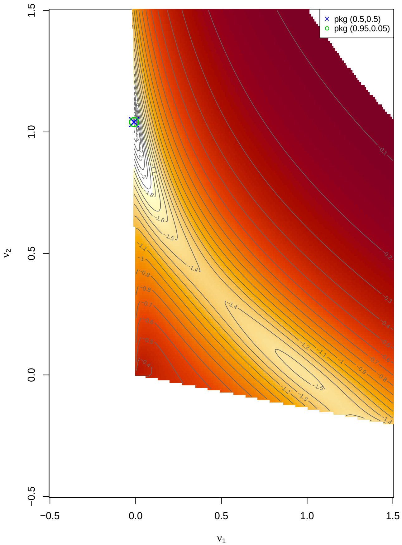
Rep 1: CUE Q(\nu)=G'W(\nu)G (log10)
