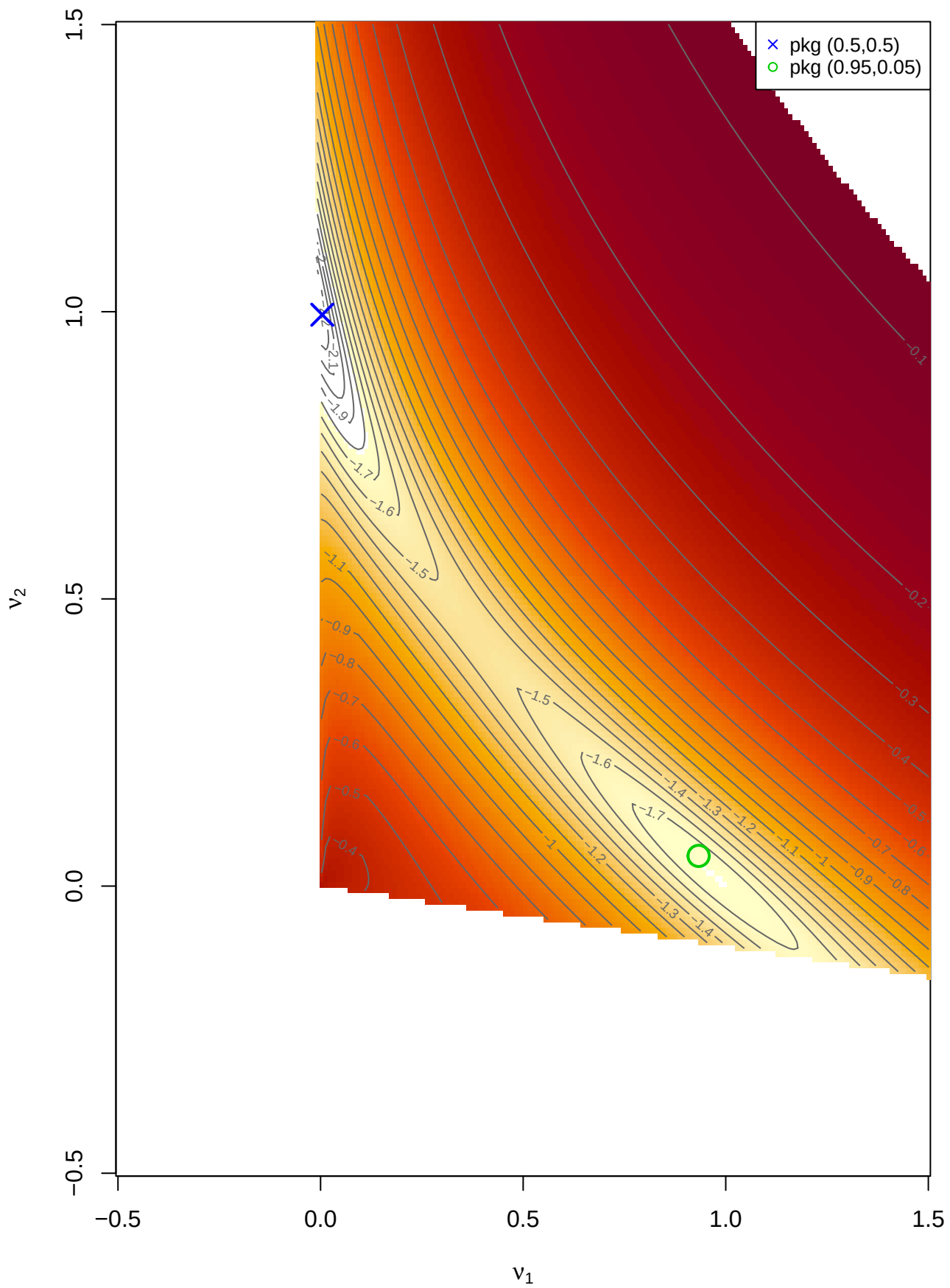
Rep 4: CUE Q(\nu)=G'W(\nu)G (log10)
