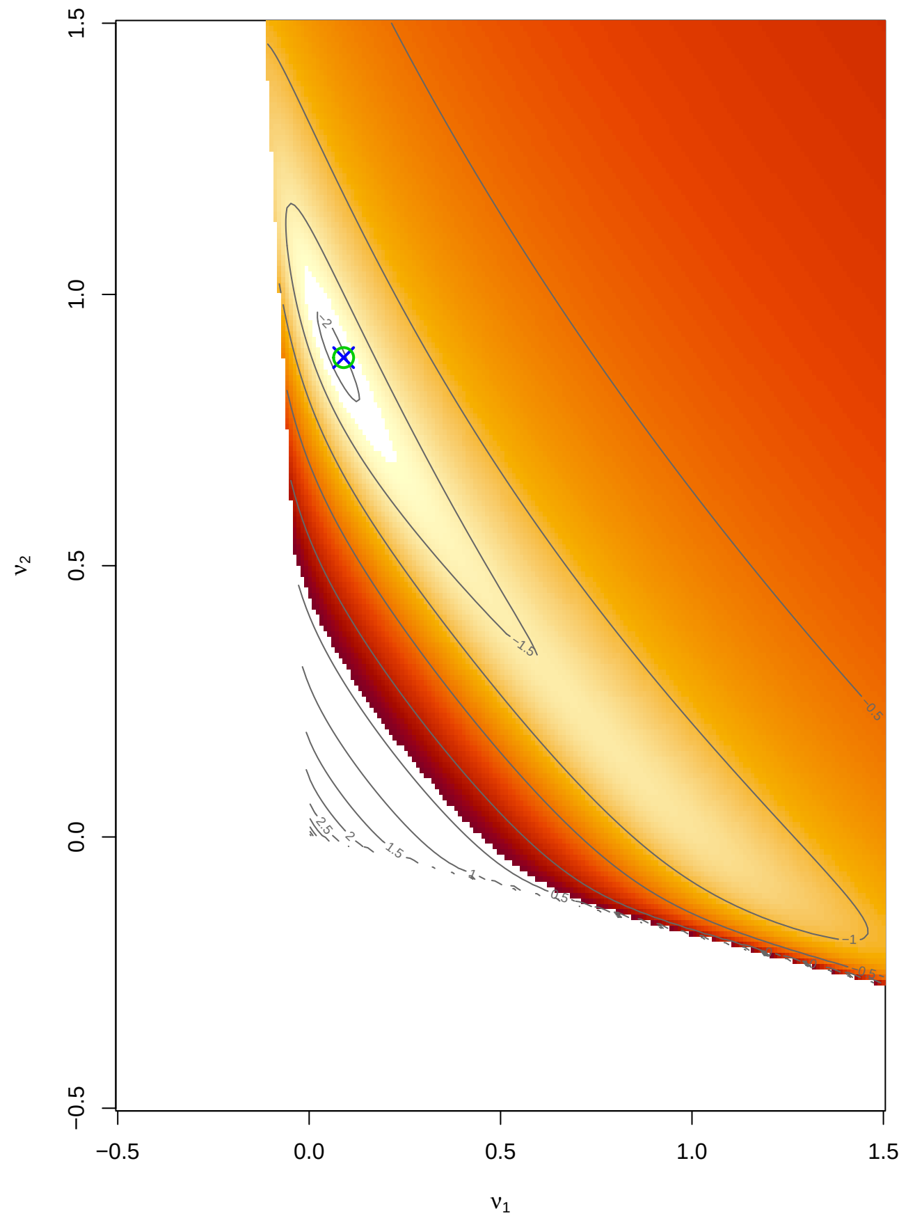
Rep 2: Fixed W=I , G'G (log10)
