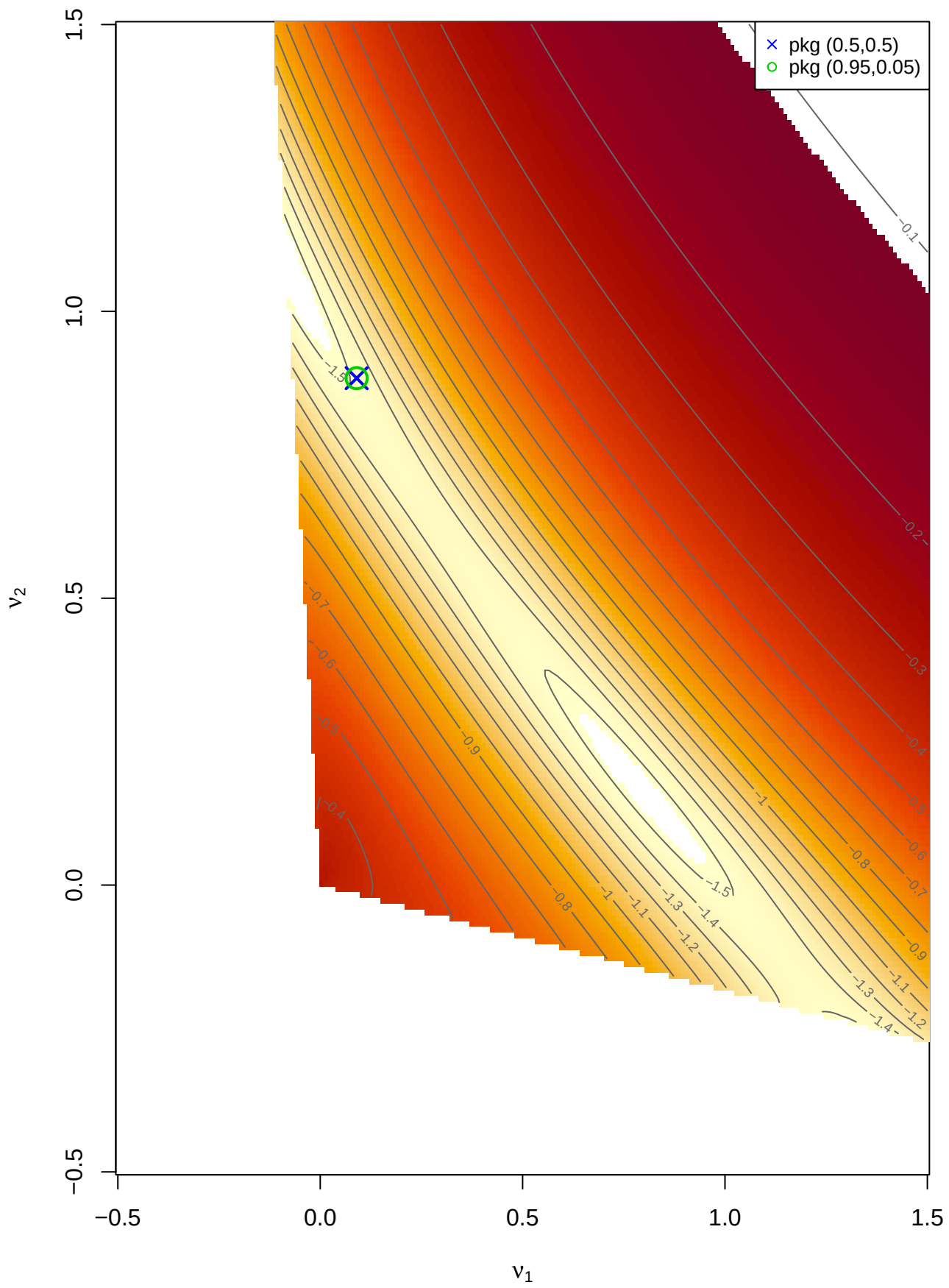
Rep 2: CUE Q(\nu)=G'W(\nu)G (log10)
