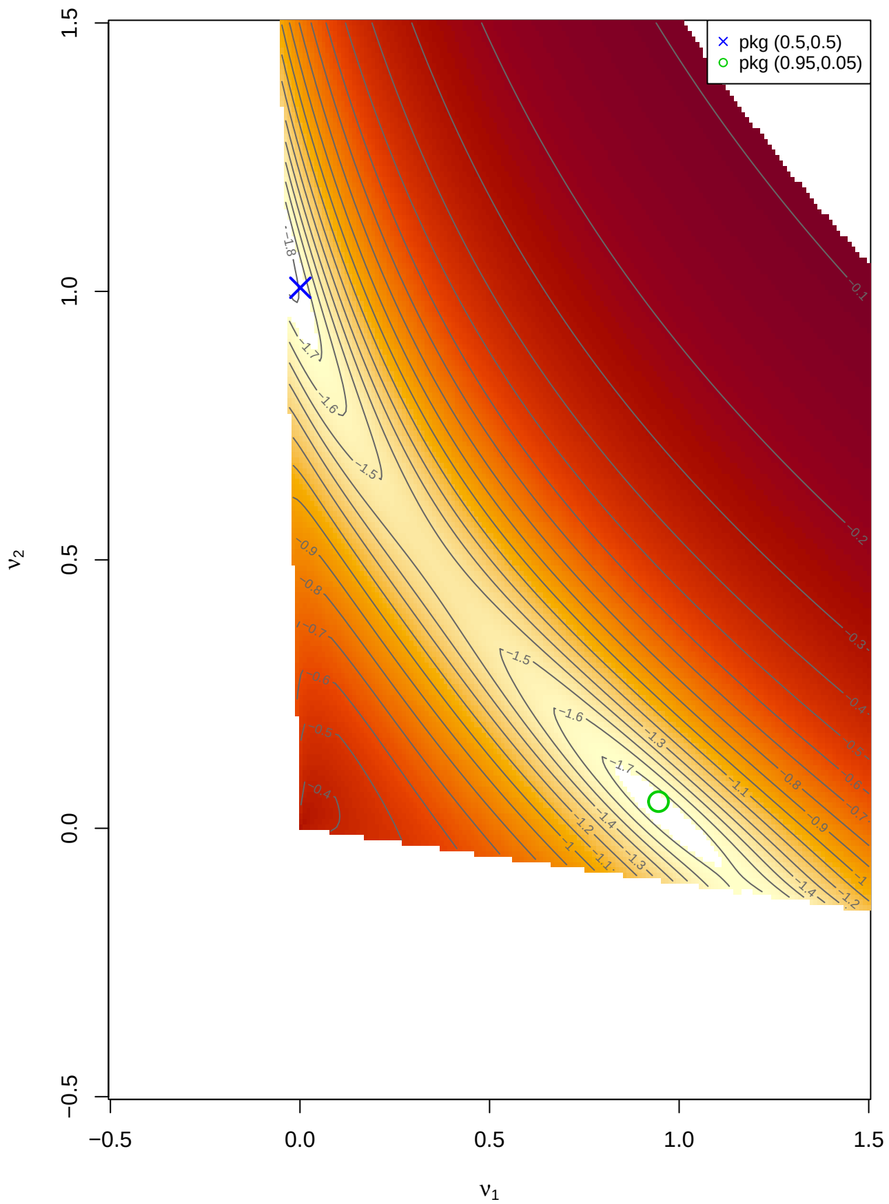
Rep 5: CUE Q(\nu)=G'W(\nu)G (log10)
