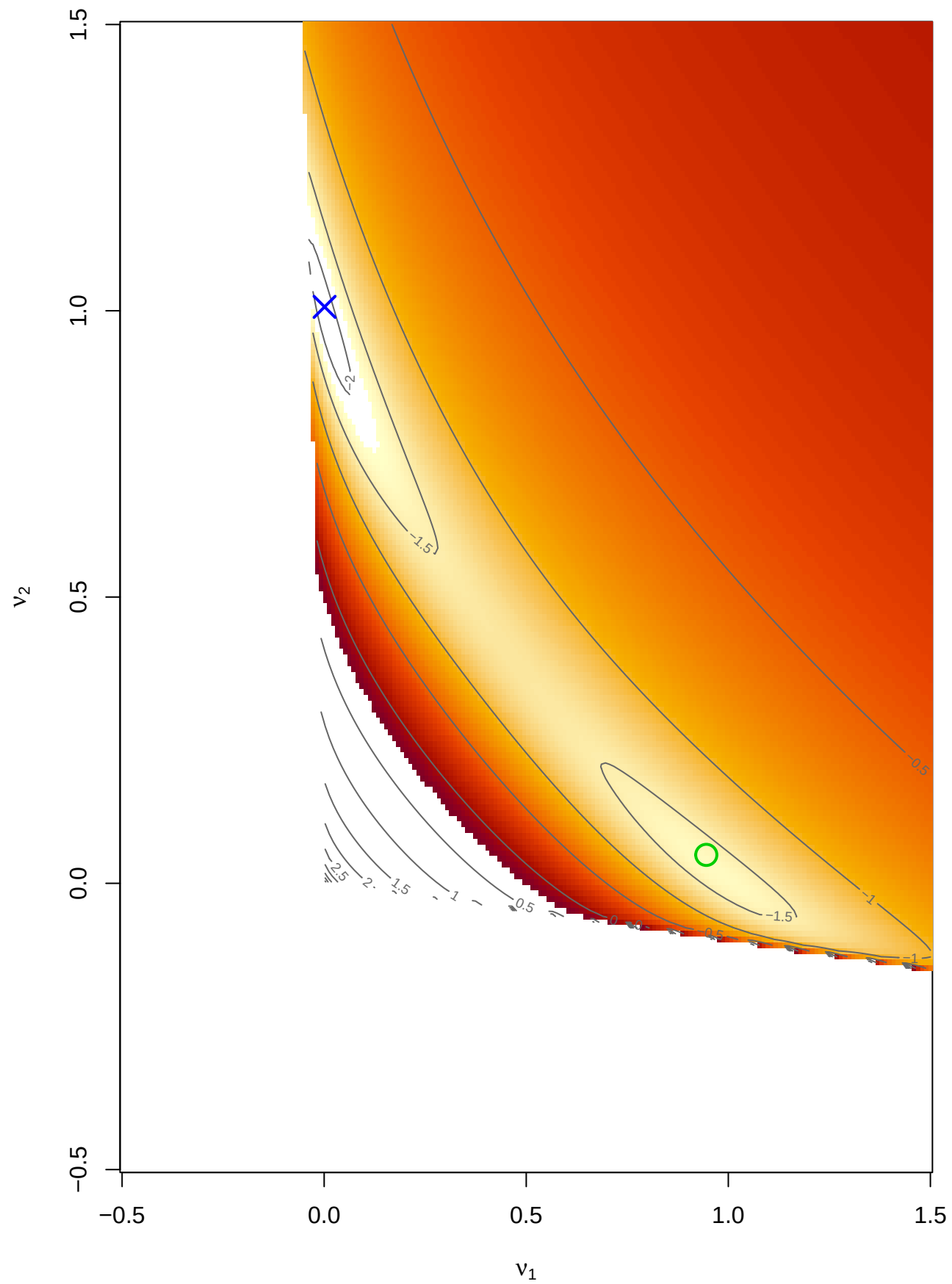
Rep 5: Fixed W=I , G'G (log10)
