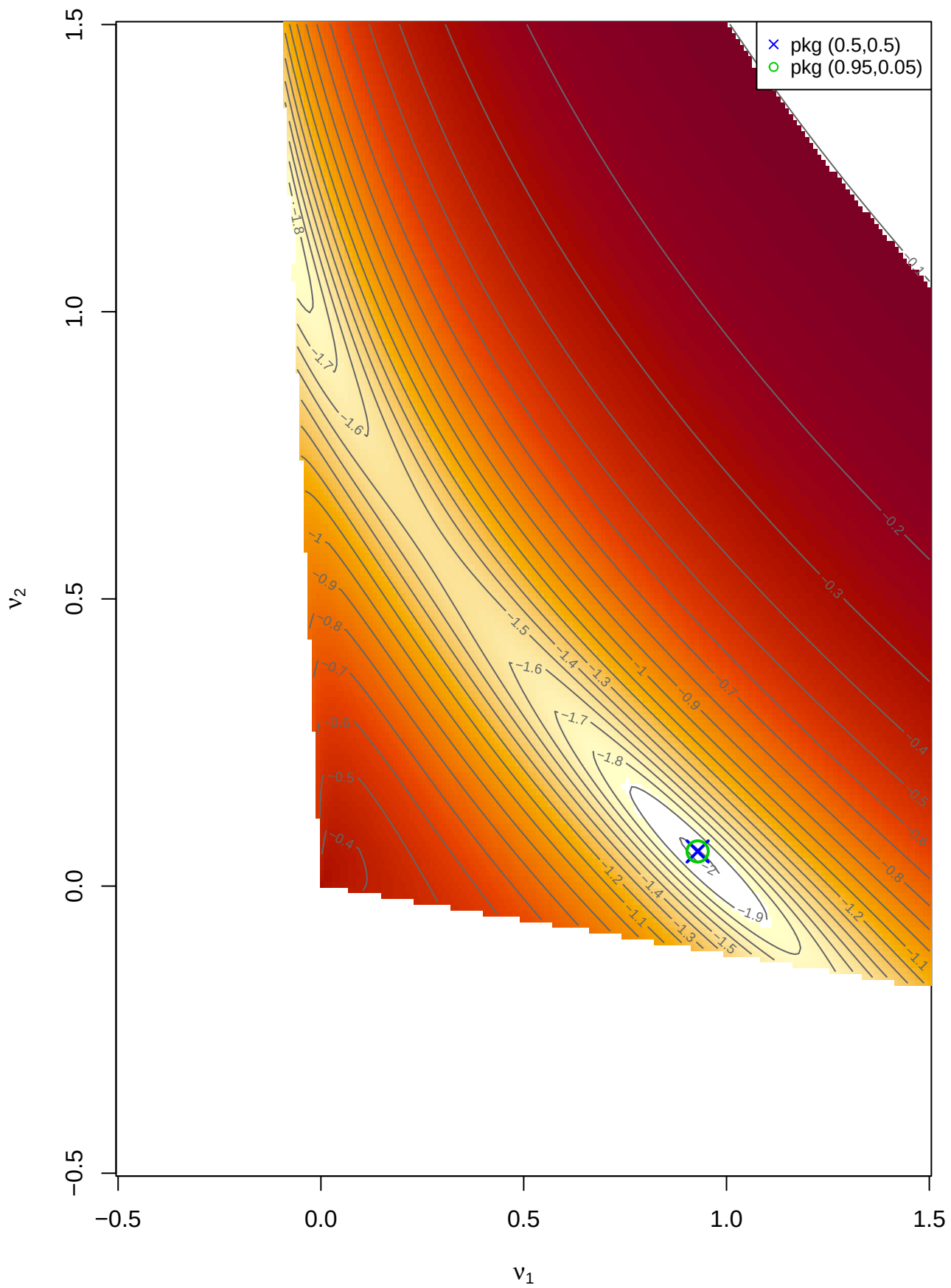
Rep 3: CUE Q(\nu)=G'W(\nu)G (log10)
