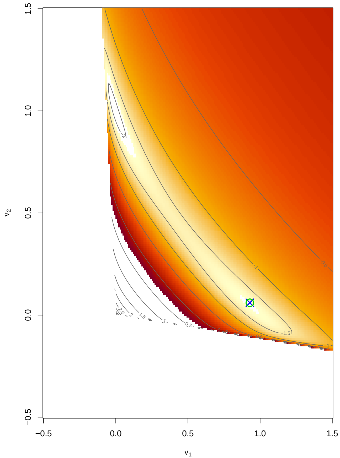
Rep 3: Fixed W=I , G'G (log10)
