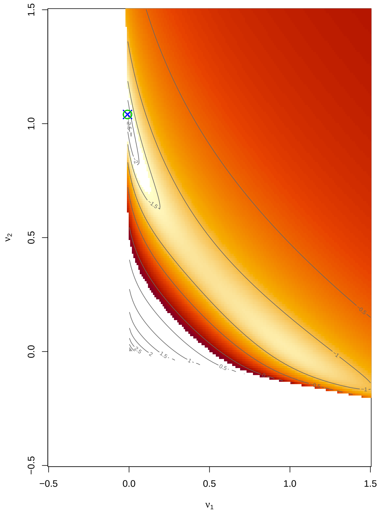
Rep 1: Fixed W=I , G'G (log10)
