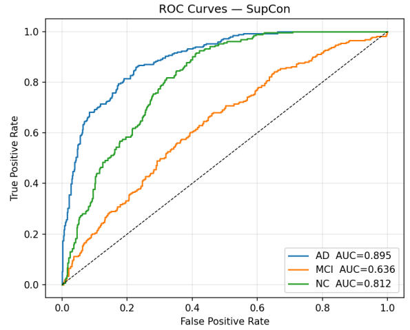
(b) ResNet-18 SupCon
