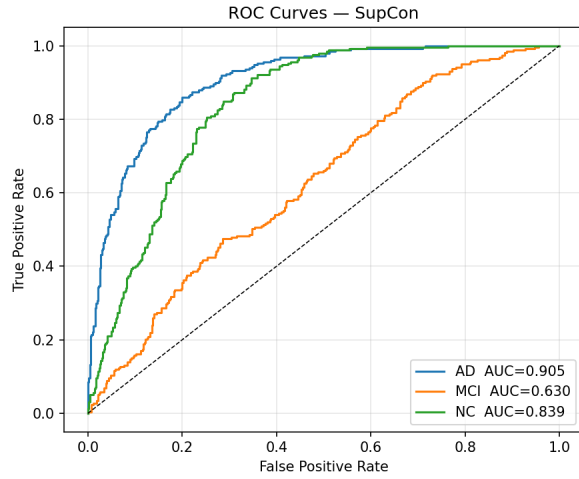
(a) ResNet-10 SupCon
