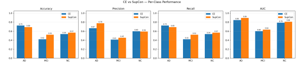
(b) ResNet-18
