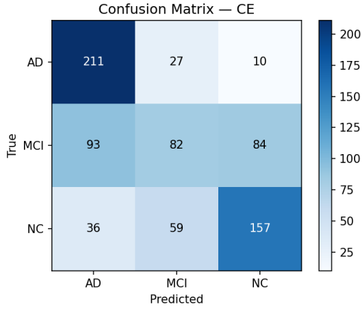
(a) ResNet-10 CE
