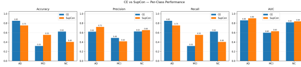
(a) ResNet-10
