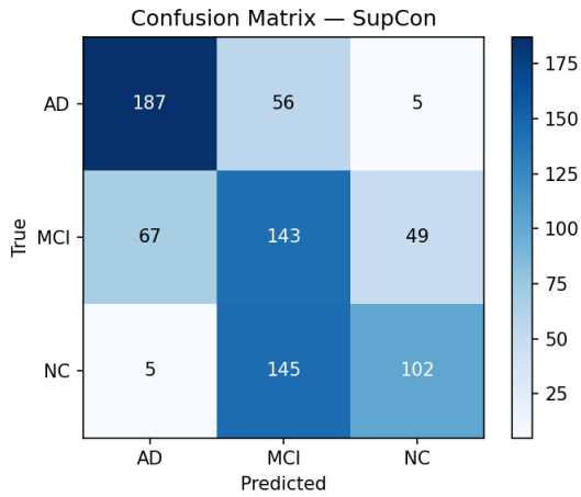
(a) ResNet-10 SupCon
