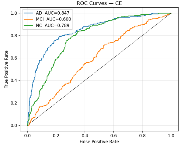
(b) ResNet-18 CE
