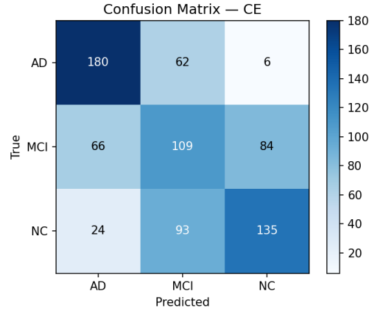
(b) ResNet-18 CE
