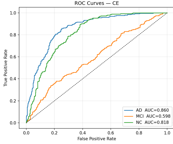
(a) ResNet-10 CE
