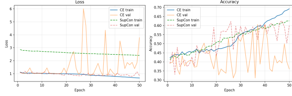
(a) ResNet-10
