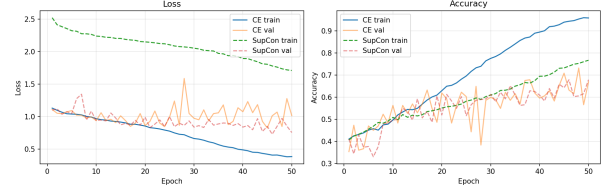
(b) ResNet-18
