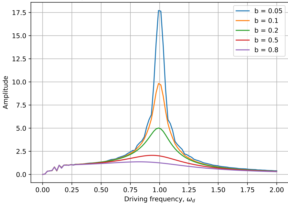
Amplitude of Resonance for Different Damping
