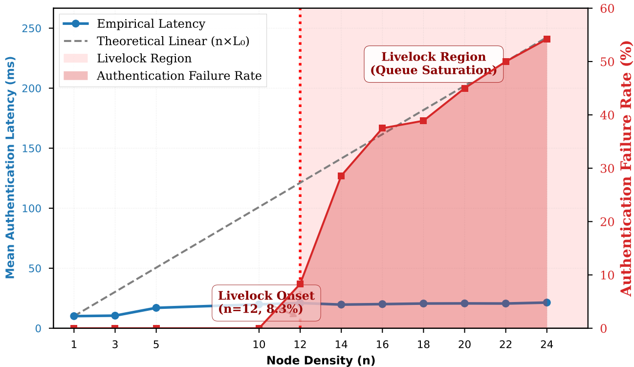
Figure 4.3: H3 Scalability & Livelock Analysis
