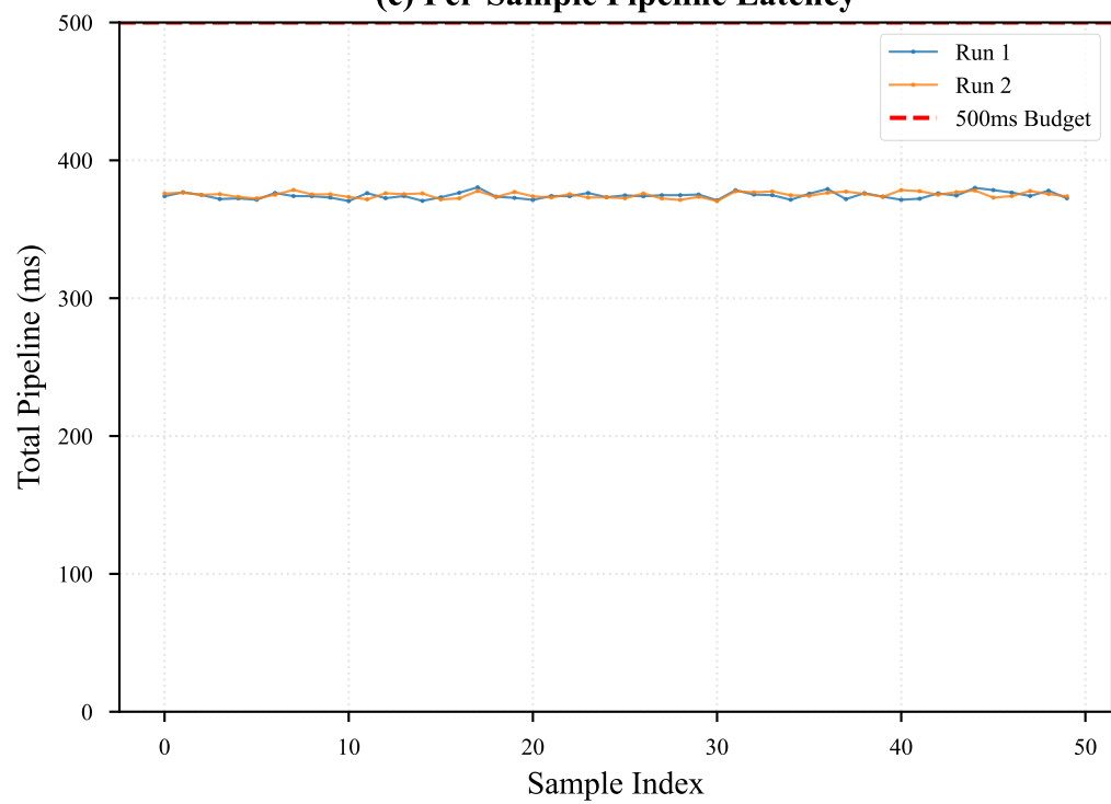
(c) Per-Sample Pipeline Latency
