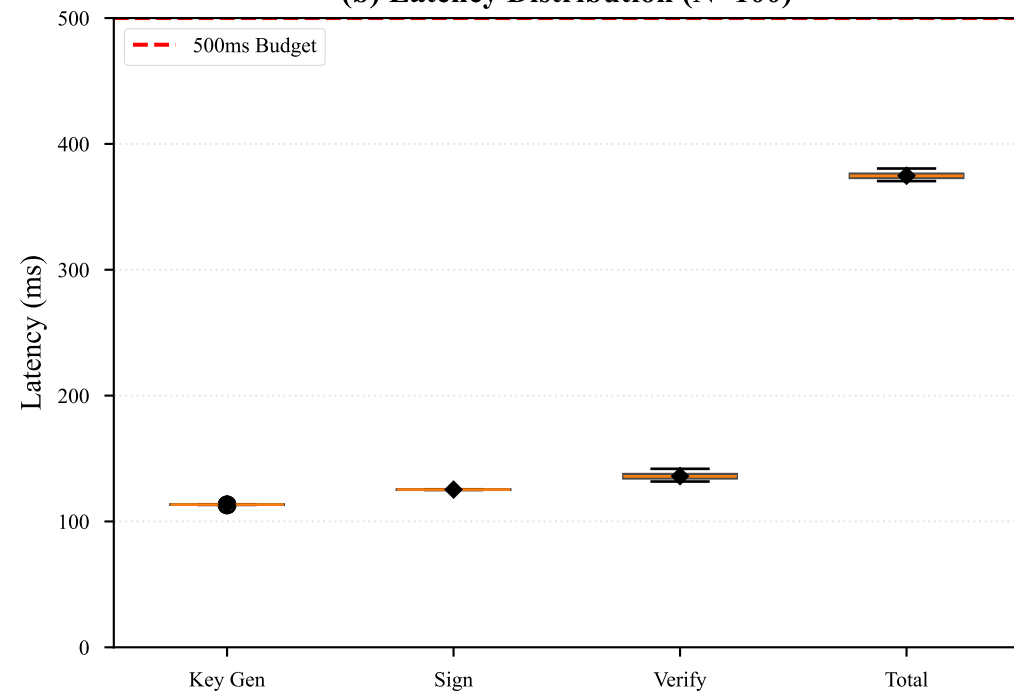
(b) Latency Distribution (N=100)
