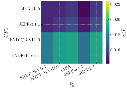
(b) The total delayed neutron yield using JEFF-3.1.1 half-lives.
