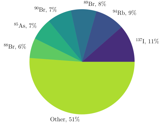
Fig. 6. The fraction of the delayed neutron yield from particular DNP groups from ENDF/B-VII.1 nuclear data. The six DNP groups with the largest delayed neutron yield contribute approximately 50% of the total delayed neutrons per fission event. The remaining 212 DNP groups provide approximately 50% of the total delayed neutron yield.
