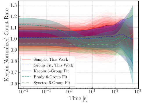
(b) The delayed neutron count rate as a function of time relative to the Keepin et al. DNP group parameter delayed neutron count rate (such that the Keepin 6-Group Fit is unity at all points in time). Comparison is made between the six DNP group parameters from this work, Brady and England, and Synetos and Williams [24, 5, 25].
