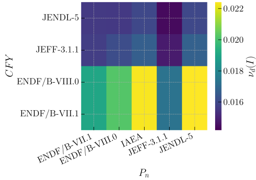
(a) The total delayed neutron yield using ENDF/B-VII.1 half-lives.
