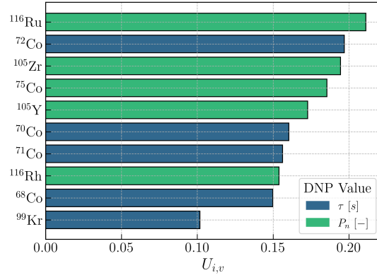
Fig. 4. The ten largest uncertainty-weighted PCCs U_{i,v} sorted by DNP and associated DNP value from JENDL-5 cumulative fission yields and IAEA \beta -delayed neutron emission database half-lives and emission probabilities.
