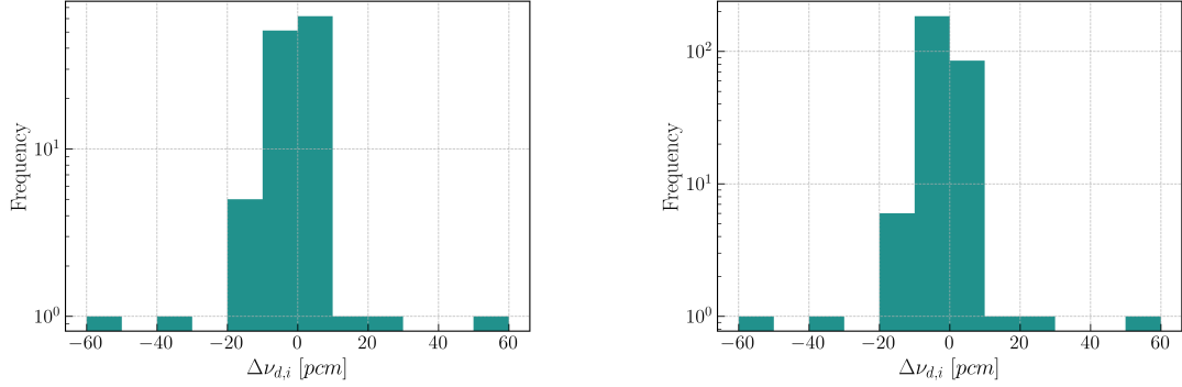
(a) The JEFF-3.1.1 \text{DNP } \nu_{d,i} minus the JENDL-5 \text{DNP } \nu_{d,i} for \text{DNPs} present in both datasets.
