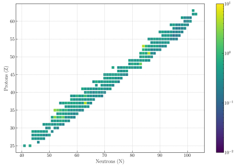
(a) The PCC_i , or total PCC , calculated for each DNP .
