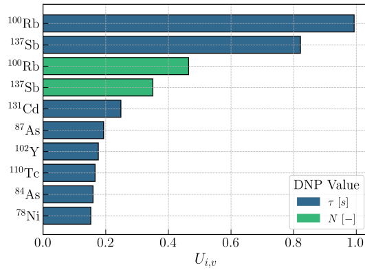
Fig. 7. The ten largest uncertainty-weighted PCCs U_{i,v} sorted by DNP and associated DNP value from JENDL-5 cumulative fission yields and IAEA beta-delayed neutron emission database half-lives and emission probabilities.
