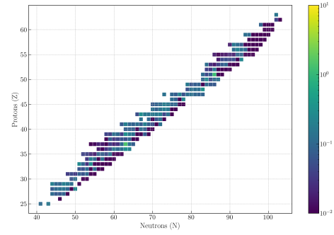
(b) The U_i , or total uncertainty-weighted PCC , for each DNP .
