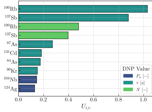
Fig. 10. The ten largest uncertainty-weighted PCCs U_{i,v} sorted by DNP and associated DNP value from JENDL-5 cumulative fission yields and IAEA beta-delayed neutron emission database half-lives and emission probabilities.
