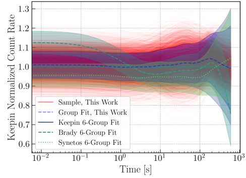
(b) The delayed neutron count rate as a function of time relative to the Keepin et al. DNP group parameter delayed neutron count rate (such that the Keepin 6-Group Fit is unity at all points in time). Comparison is made between the six DNP group parameters from this work, Brady and England, and Synetos and Williams [24, 5, 25].
