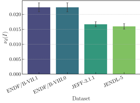
(a) The total delayed neutron yield.
