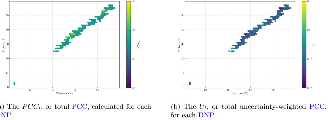
Fig. 5. Chart of nuclide plots showing the PCC s and uncertainty-weighted PCC s using JENDL-5 cumulative fission yields and IAEA beta-delayed neutron emission database emission probabilities and half-lives.
