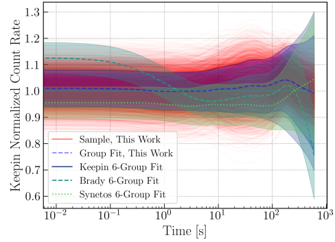
(b) The delayed neutron count rate as a function of time relative to the Keepin et al. DNP group parameter delayed neutron count rate for DNP six group parameters from this work, Brady and England, and Synetos and Williams [23, 5, 24].
