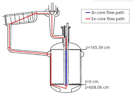
Fig. 1. The flow path and bounds for the in-core region of the MSRE, overlayed on the MSRE loop diagram from [14].
