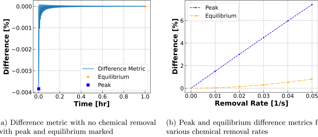
Fig. 6. ^{135}\text{Xe} chemical removal rate difference metrics in the MSRE.
