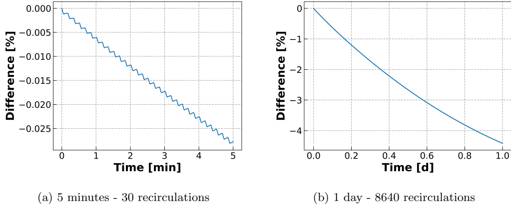
Fig. 5. ^{135}\text{Xe} difference metrics in a toy model with 5 second in-core and ex-core residence times over different periods of time.
