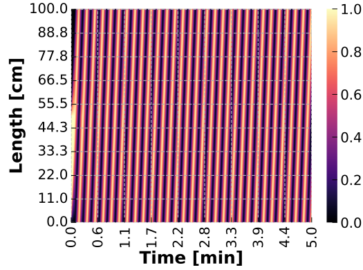
Fig. 4. Relative maximum concentration at each time step of ^{135}\text{Xe} in a toy model with 5 second in-core and ex-core residence times and a square wave power oscillation.
