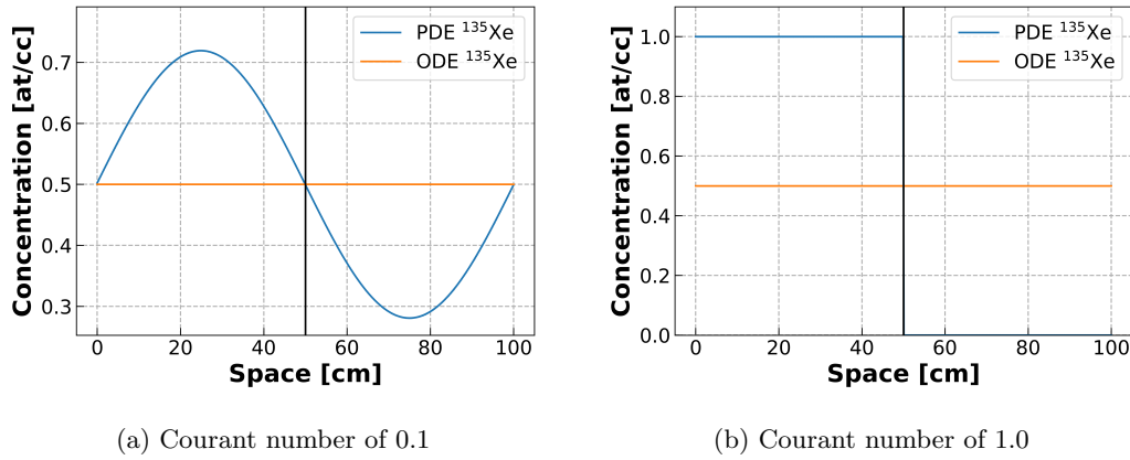
Fig. 2. Concentration for a simple test case in a 100 cm long channel with a flow rate of 10 cm/s after 5 minutes with no source or loss terms and an initial concentration in the first 50% of the loop.
