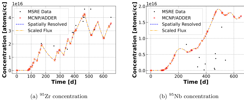
Fig. 3. Concentrations over time in the Molten Salt Reactor Experiment with no chemical removal.
