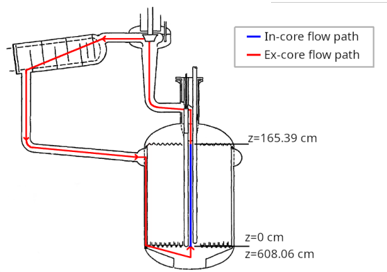
Fig. 1. The flow path and bounds for the in-core region of the MSRE, overlaid on the MSRE loop diagram from [14].
