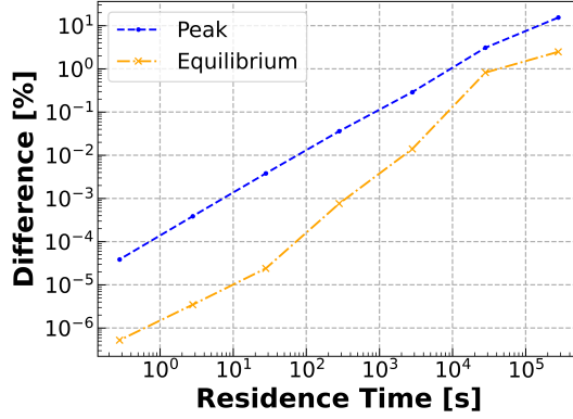
Fig. 7. Peak and equilibrium difference metrics for various primary loop residence times in the MSRE for ^{135}\text{Xe} .
