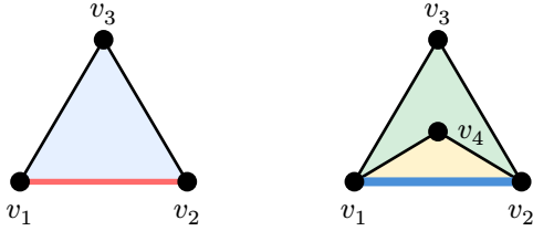
2-simplex \sigma = \{v_1, v_2, v_3\} 1-simplex \tau = \{v_1, v_2\} facet: \{v_1, v_2\} cofaces: \{v_1, v_2, v_3\} , \{v_1, v_2, v_4\}
