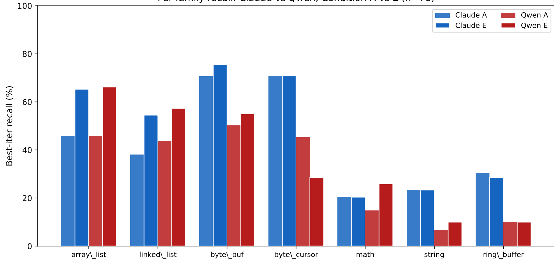
Per-family recall: Claude vs Qwen, Condition A vs E (n=76)
