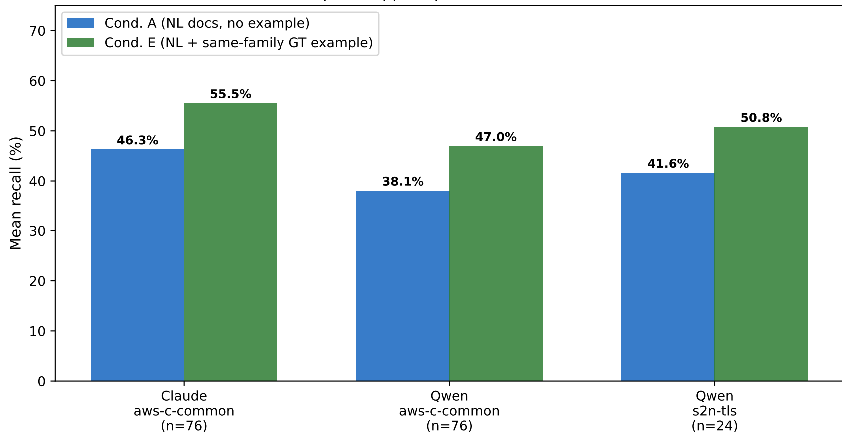
Few-shot GT Example (+9pp) Replicates Across Libraries and Models
