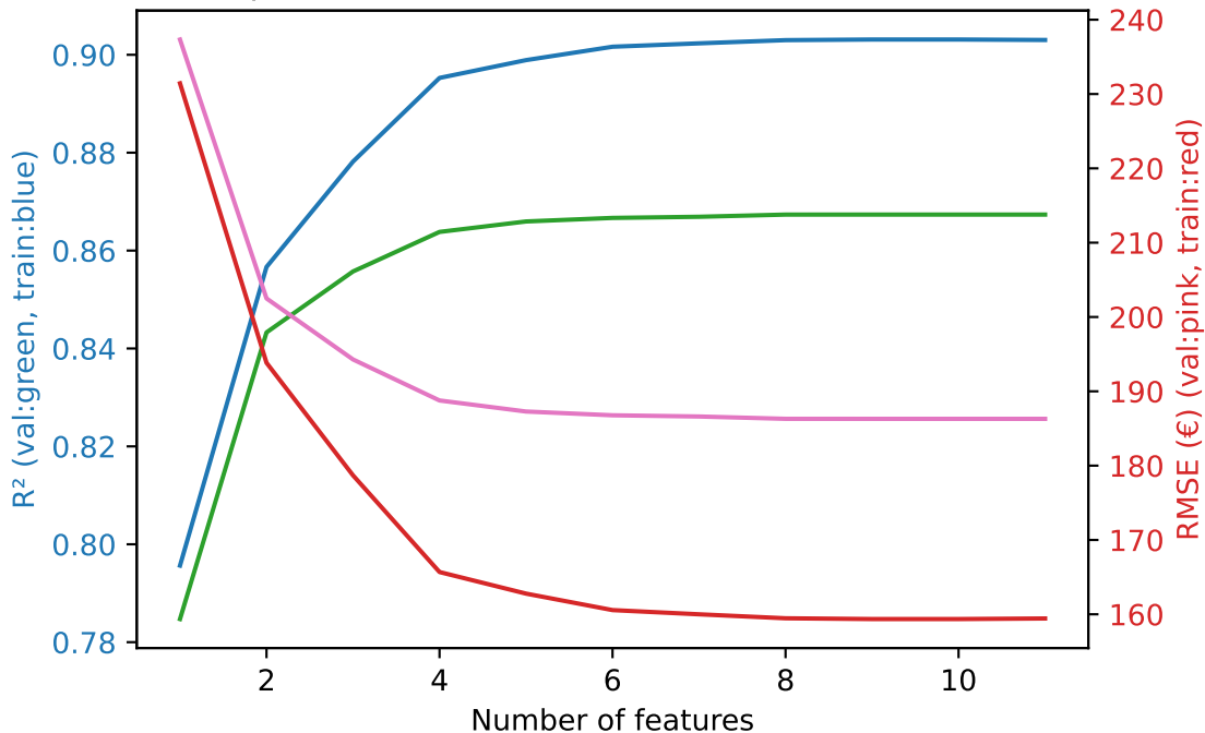
Model performance (validation) vs. number of features
