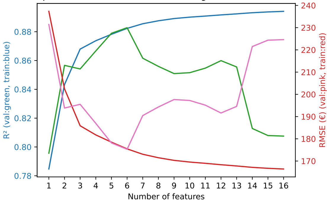
Model performance (validation & training) vs. number of features
