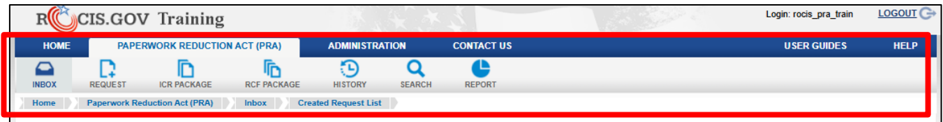
Figure 20: Navigation Toolbar
