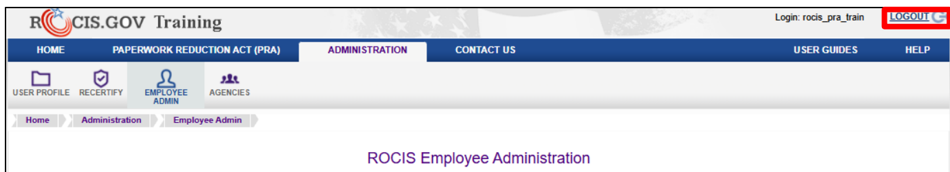
Figure 6: 'Logout' Link
