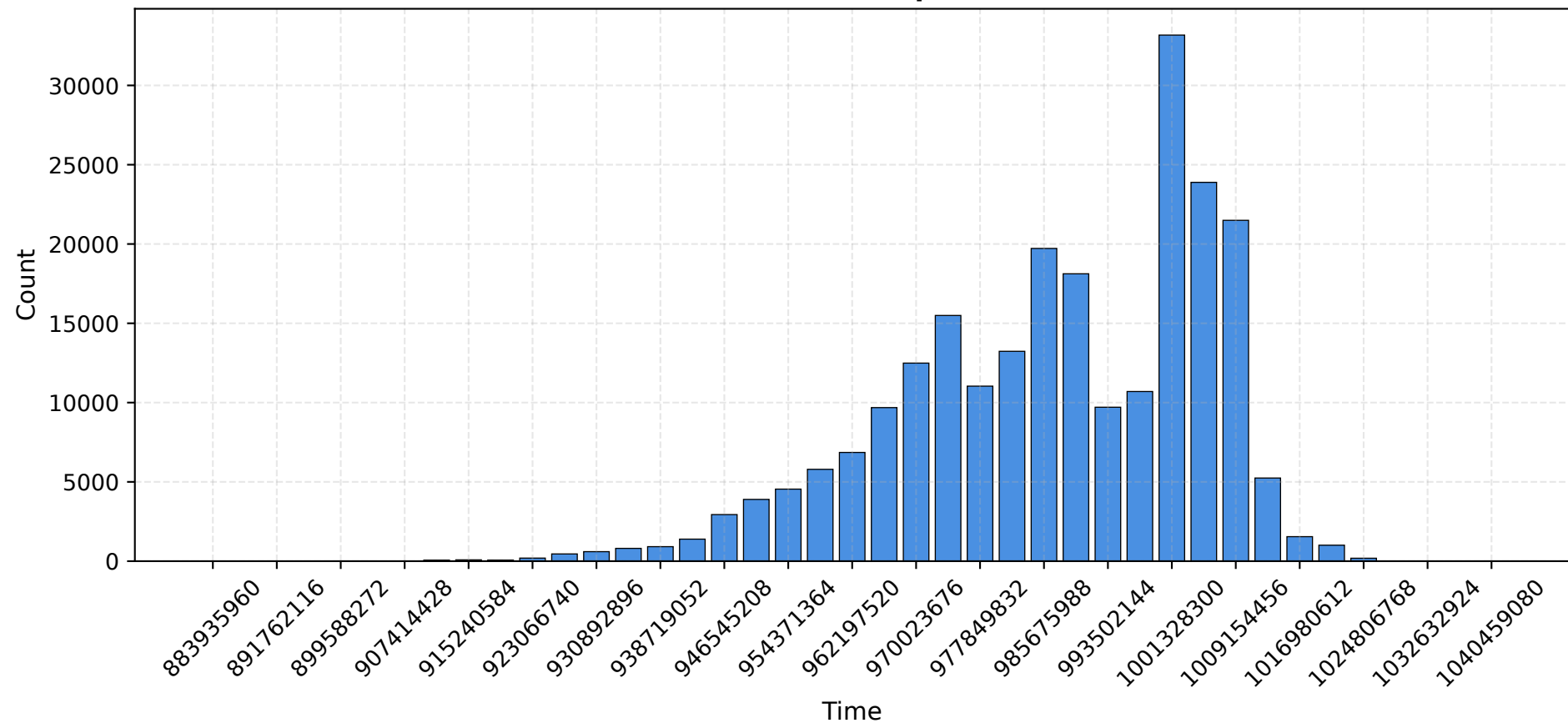
Arches Distribution email Enron - Time span: [883935960 - 1040459085]
