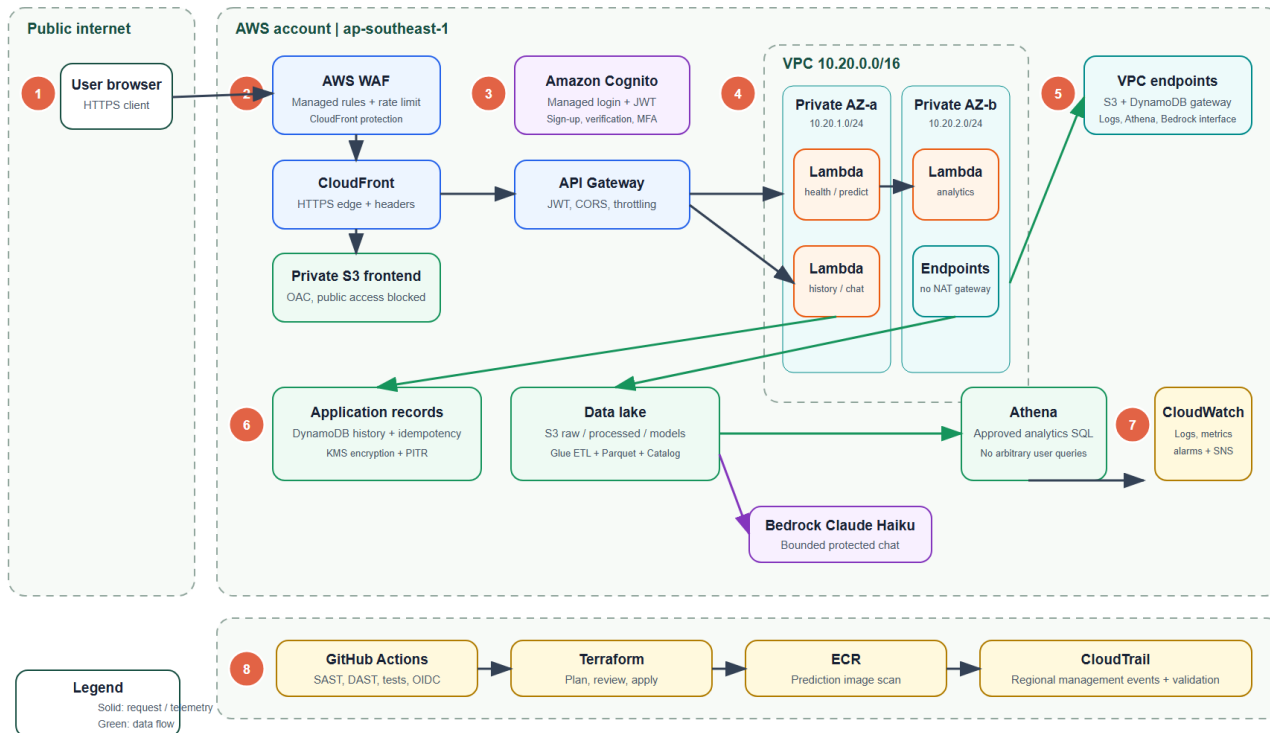
Figure 1. Current deployed serverless architecture and trust boundaries.
