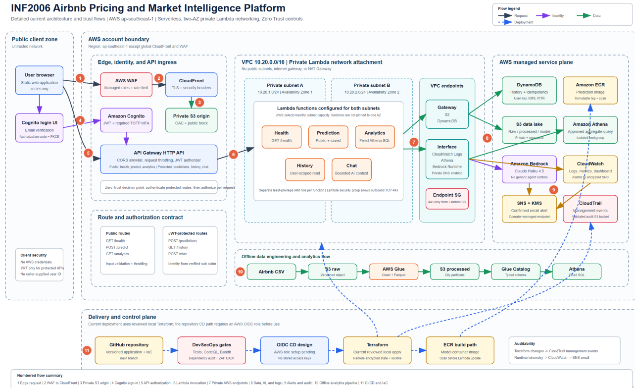
Figure 1. Current deployed serverless architecture and trust boundaries.
