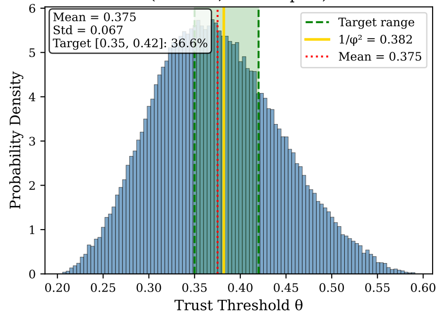
Game Theory \theta Distribution (n = 100,000 samples)
