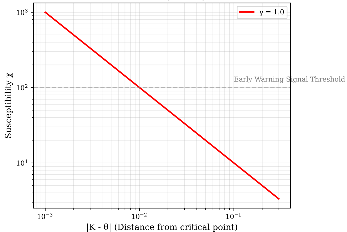
B) Susceptibility Divergence
