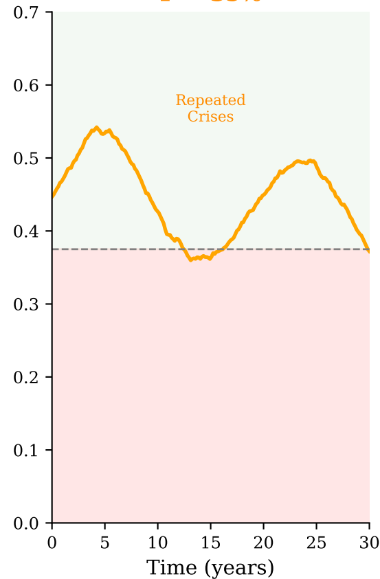
Scenario C: Unstable P = 35%
