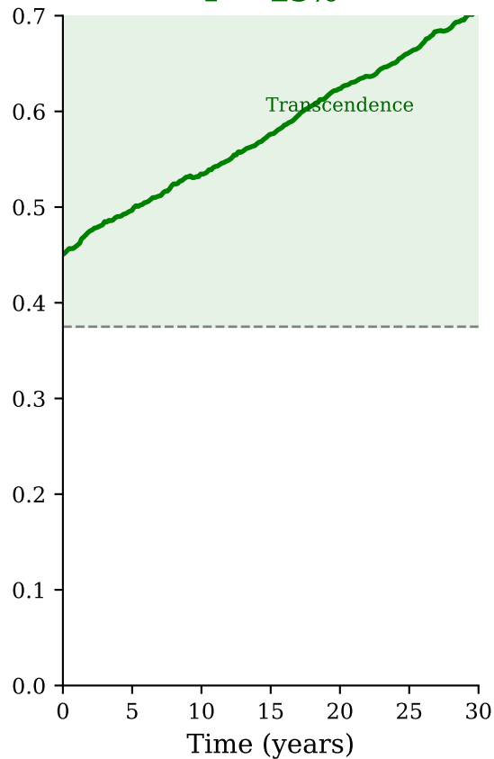
Scenario B: Enhancement P = 25%
