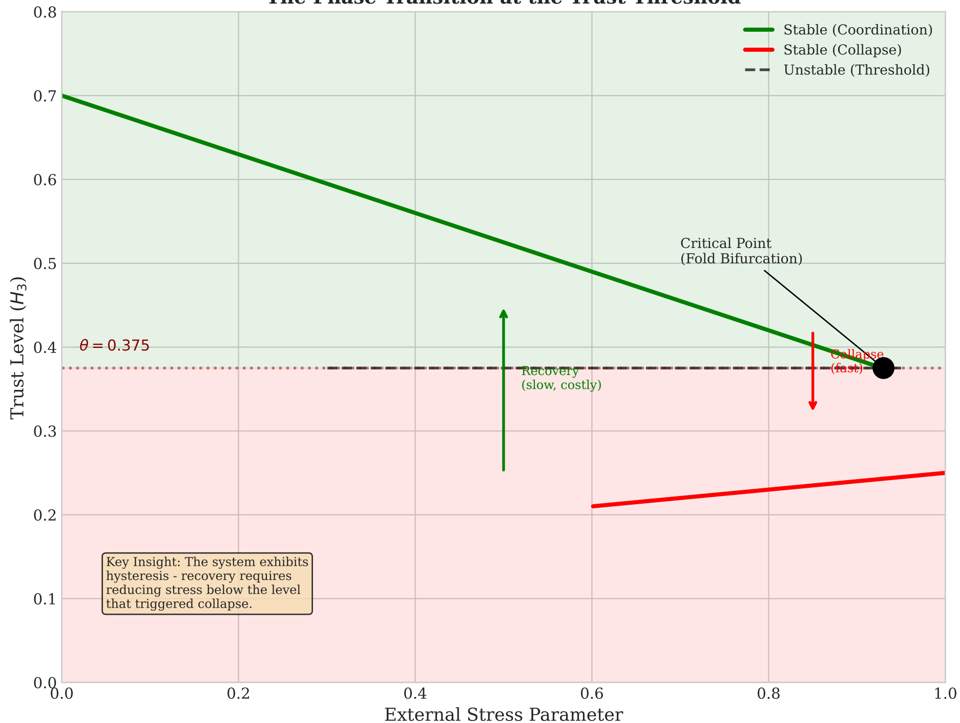
Figure S3: Bifurcation Structure of Civilizational Collapse The Phase Transition at the Trust Threshold
