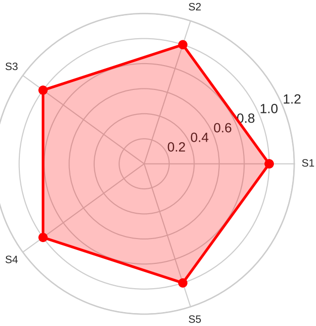
South Africa H_3=0.41 , 4/5 signatures
