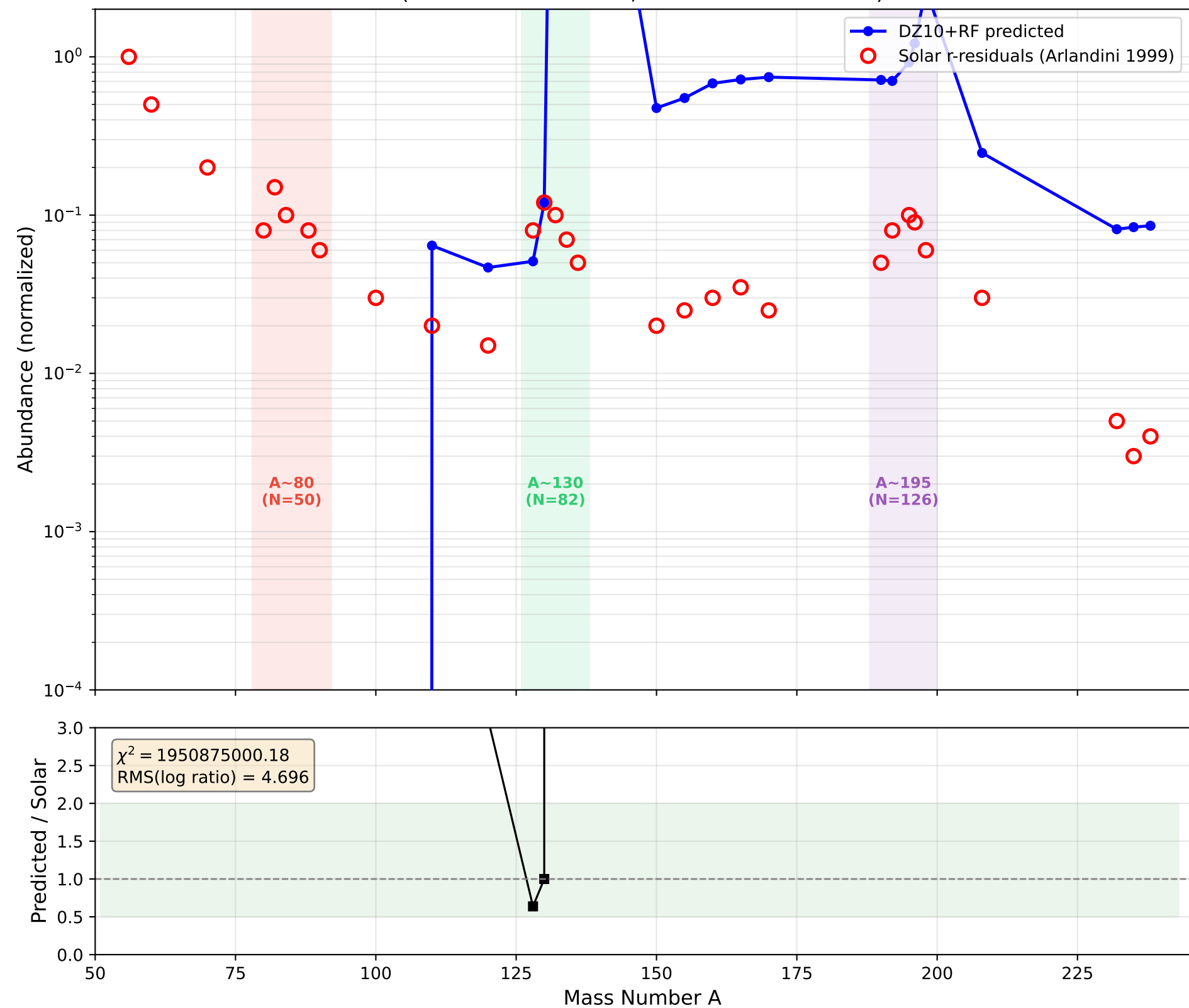
R-Process Abundances vs Solar R-Residuals (Arlandini et al. 1999, normalized at A=130)
