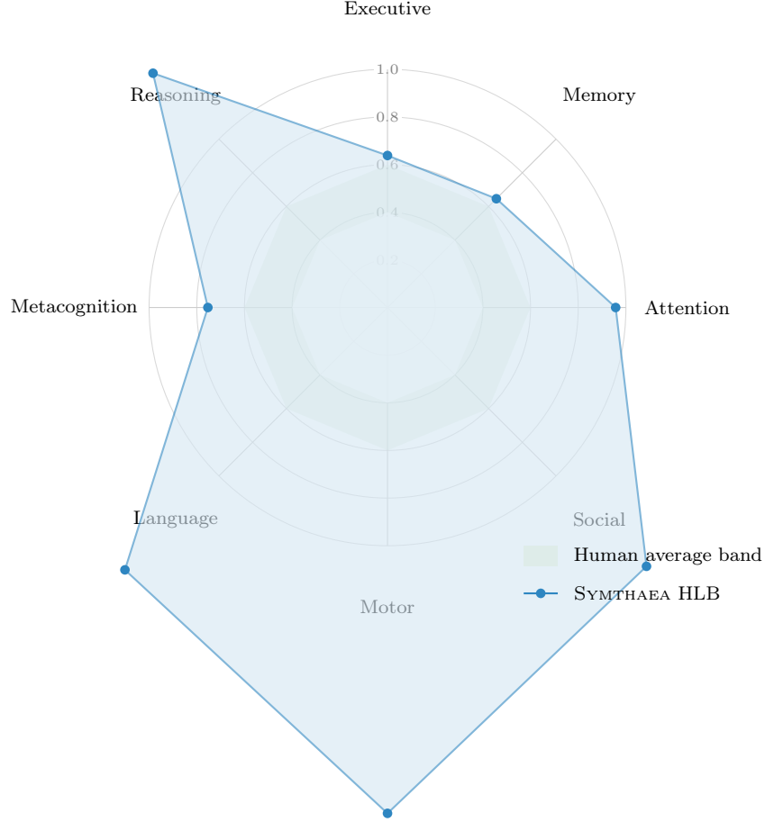
Figure 7: Eight-domain cognitive profile of the SYMTHAEA Holographic Liquid Brain, generated from benchmark data. The green band represents the human average range (normalized 0.4–0.6). Domain scores loaded from cognitive_profile.csv .
