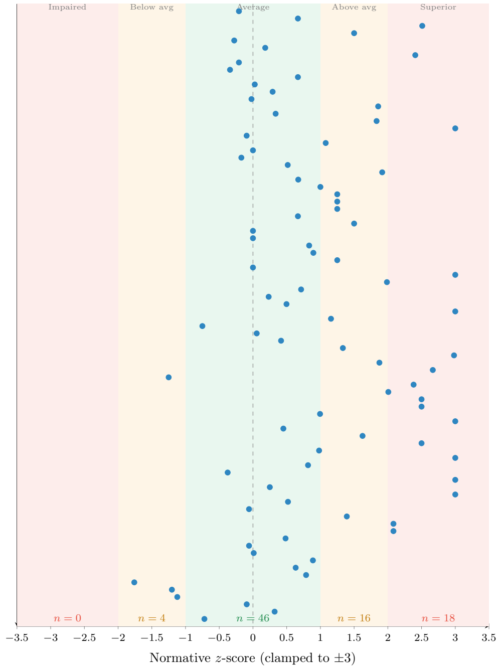
Figure 8: Forest plot of normative z-scores for 84 benchmarks with matched human baselines (z-scores clamped to \pm 3 for readability). Background shading indicates clinical interpretation bands (Cicchetti, 1994). Band counts: 46 Average ( |z| \leq 1 ), 16 Above Average, 4 Below Average, 18 Superior ( z > 2 ), 0 Impaired ( z < -2 ). Data loaded from normative_zscores.csv .
