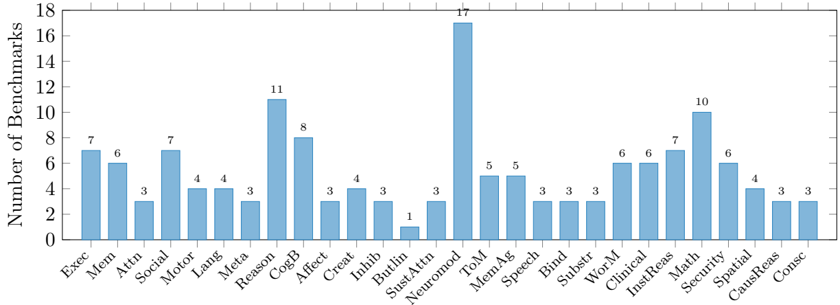
Figure 3: Benchmark count by domain across all 28 domain categories. The neuromodulator evaluation framework (17 benchmarks) is the largest single domain, reflecting its novel contribution. Reasoning (11), Mathematics (10), CogBench (8), InstitutionalReasoning (7), and Social (7) provide additional depth. Eight domains map to the cognitive profile radar chart; the remainder are specialized sub-batteries including Clinical, Security (FHE), Speech, Binding, Substrate, Spatial, CausalReasoning, Consciousness, and WorM domains.
