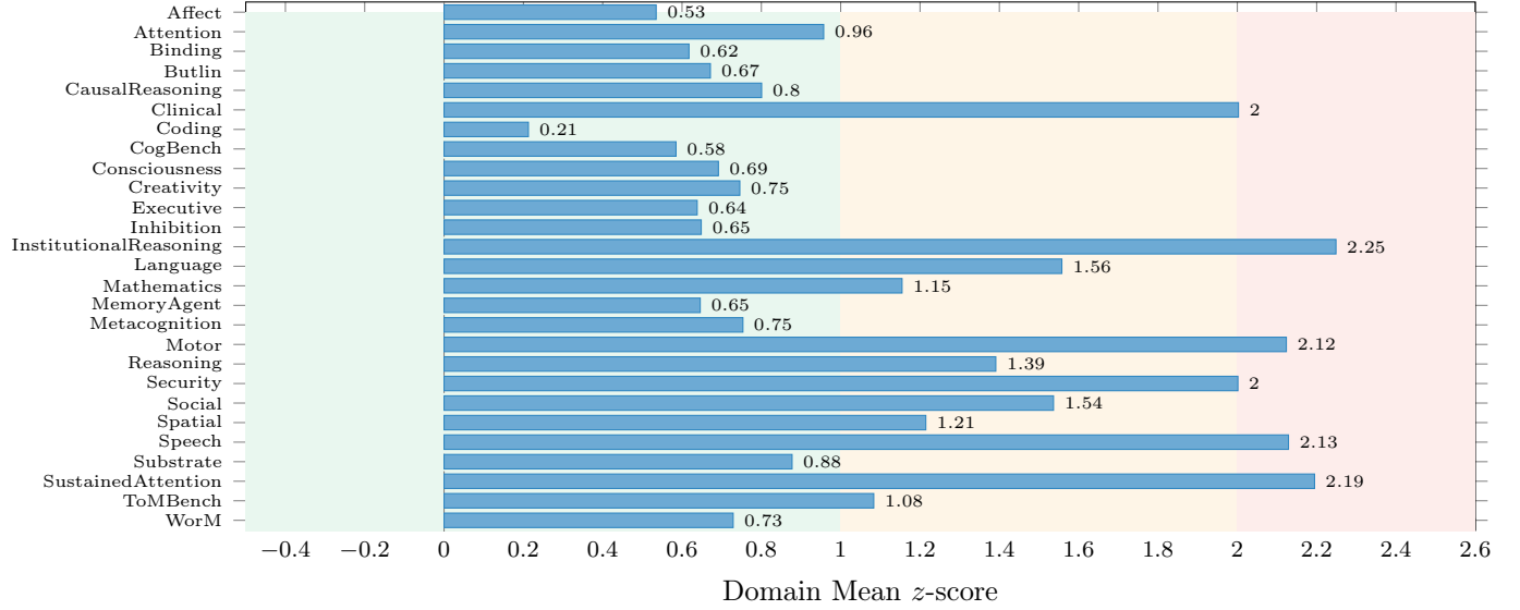
Figure 6: Complete 27-domain signature profile of the SYMTHAEA HLB, showing domain-level mean z -scores. Background shading: green = Average ( |z| \leq 1 ), yellow = Above Average/Strong ( 1 < z \leq 2 ), red = Exceptional ( z > 2 ). All 27 domains fall above the human population mean ( z = 0 ). The characteristic signature—exceptional sustained attention, motor, and speech; strong reasoning and social cognition; average executive function and affect—reveals architectural biases that distinguish HLB systems from both human cognition and prompt-based LLMs. Data from cognitive_profile.csv .
