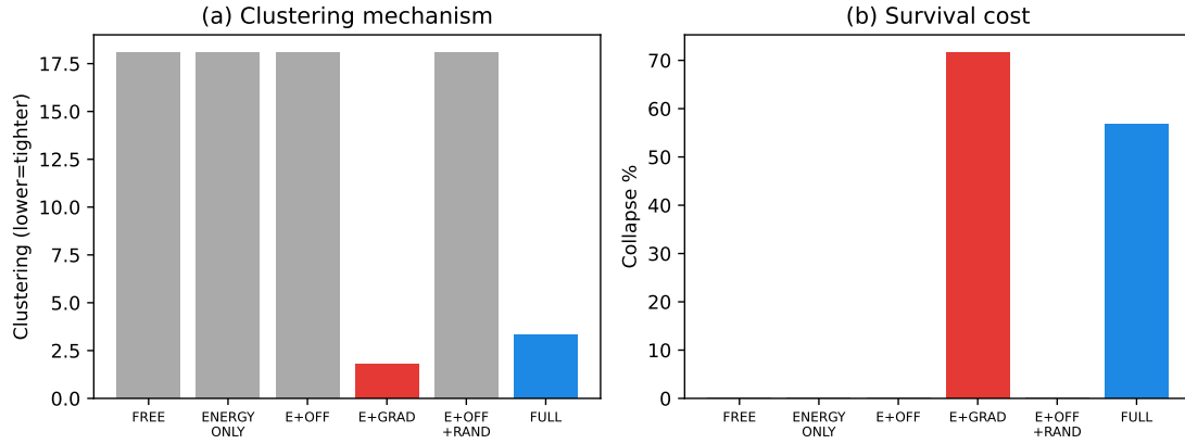
Figure 1: Ablation study (re-verified with overhauled engine). (a) Only conditions with FEP gradient cluster tightly ( < 4 ). (b) Gradient without offloading kills 72% of agents. The FEP gradient is the clustering mechanism; epistemic offloading is the survival mechanism.
