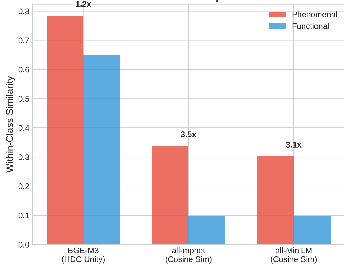
A. Cross-Model Replication
