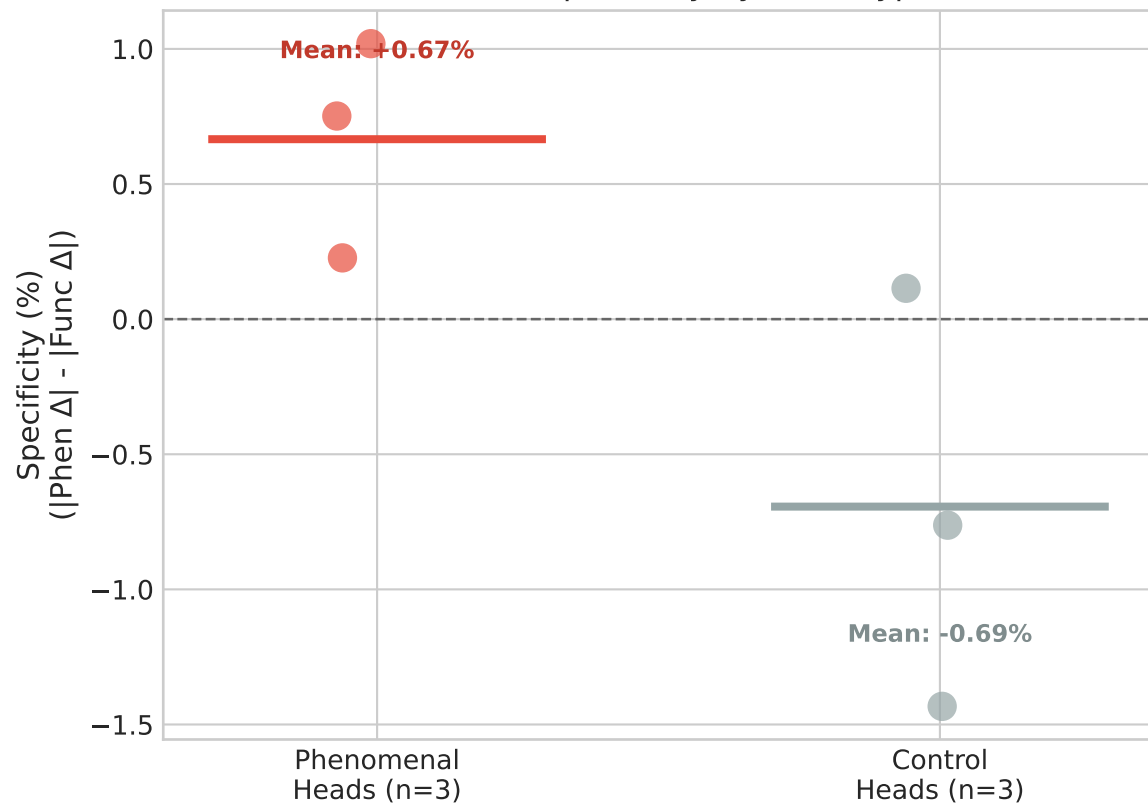
B. Causal Specificity by Head Type
