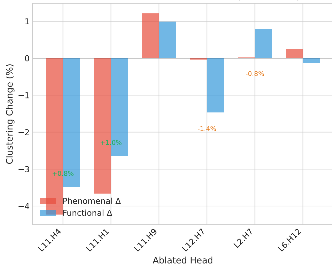
A. Effect of Head Ablation on Concept Clustering
