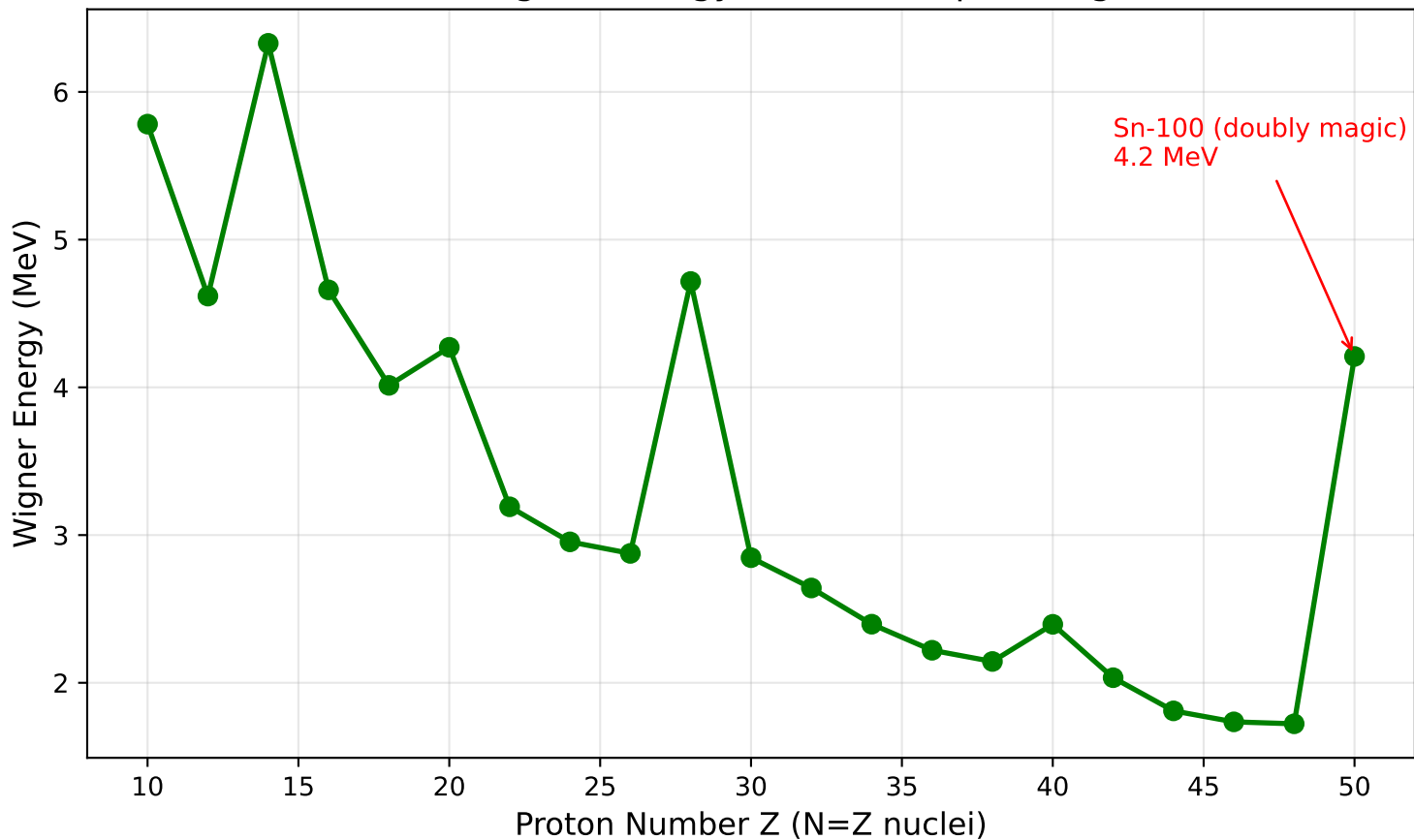
N=Z Wigner Energy (Isoscalar np Pairing)
