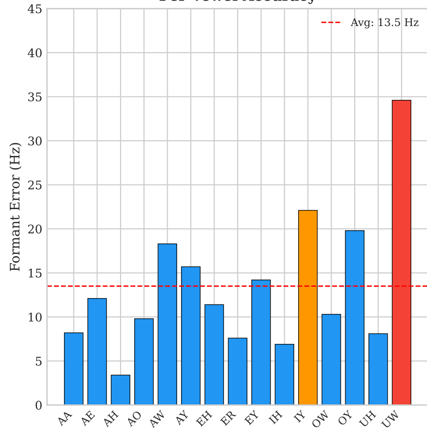
Per-Vowel Accuracy
