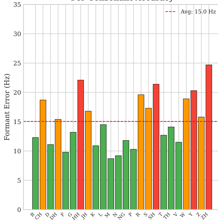
Per-Consonant Accuracy
