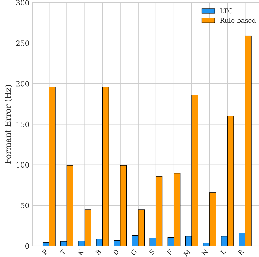
Per-Consonant Accuracy
