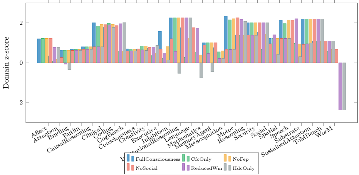
Figure 9: Ablation comparison across six presets and 27 cognitive domains. HdcOnly (Cohen’s d = 0.61 ) produces the largest overall deficit, with WorM ( \Delta = 3.09 ), Language ( \Delta = 2.51 ), and Inhibition ( \Delta = 2.10 ) most affected. ReducedWm selectively devastates WorM ( \Delta = 3.09 ) while leaving other domains largely intact. Several domains ( InstitutionalReasoning , CausalReasoning , Security , SustainedAttention , ToMBench ) are ablation-invariant ( \eta^2 = 0.000 ), reflecting reliance on structural HDC operations unaffected by encoding noise. Data loaded from ablation_domains.csv .
