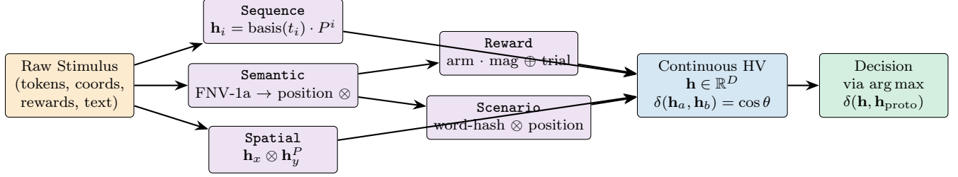
Figure 2: HDC stimulus encoding pipeline. Raw stimuli are converted to continuous hypervectors via five adapter types using binding ( \otimes ), bundling ( \oplus ), and permutation ( P ). All modalities share a common \mathbb{R}^D space where cosine similarity enables cross-modal comparison. Decisions use prototype matching via arg max similarity.
