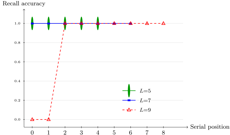
Figure 7: Serial position curves for three list lengths. Lists within WM capacity ( L=5, 7 ) show perfect recall at all positions. At L=9 (exceeds capacity by 2), FIFO eviction eliminates the two oldest items (positions 0–1), producing a sharp primacy deficit while preserving recency—the expected pattern for a capacity-limited FIFO buffer.
