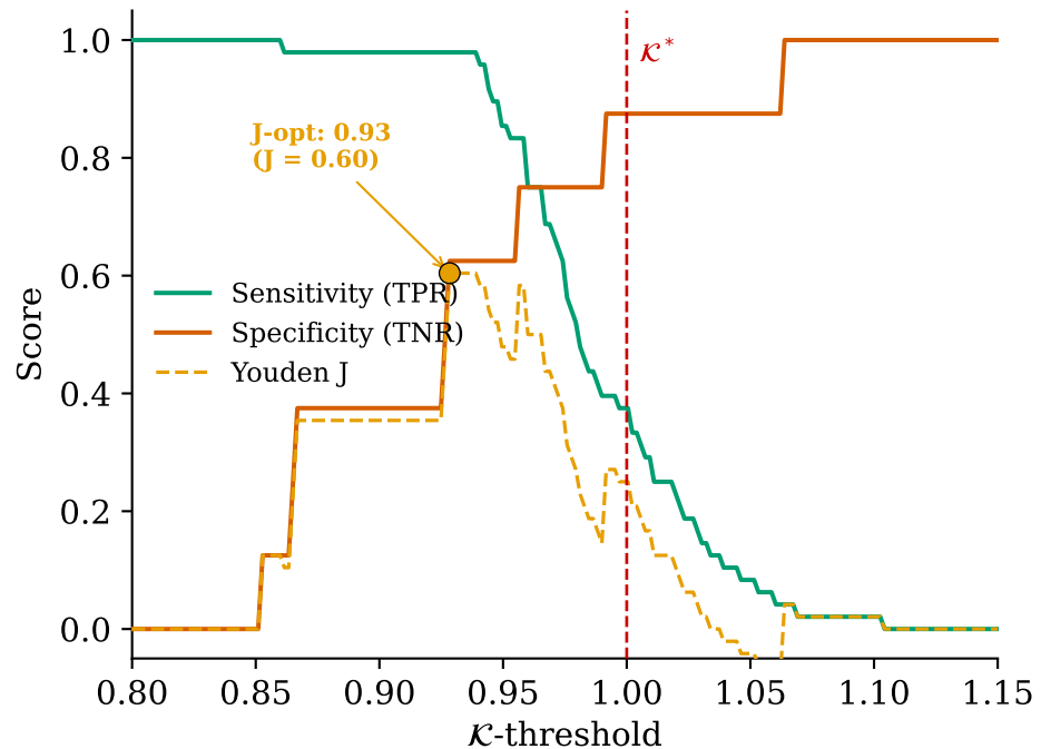
(B) Sensitivity / Specificity / Youden J
