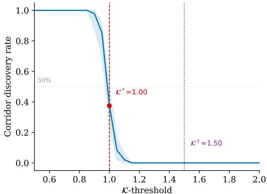
(A) Discovery rate vs threshold
