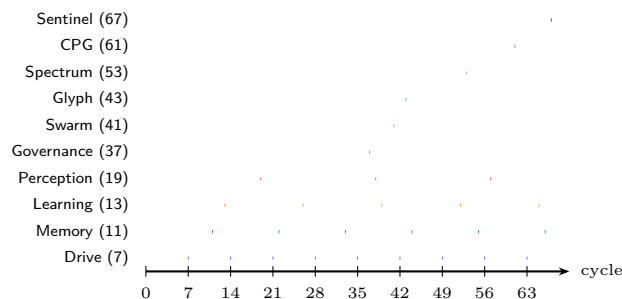
Figure 12.1: Co-prime manager activation timeline over 70 cognitive cycles. Each dot marks a cycle where that manager activates. The co-prime intervals ensure no two managers with intervals p and q coincide more frequently than every p \cdot q cycles, preventing phase-locking and distributing computational load.
