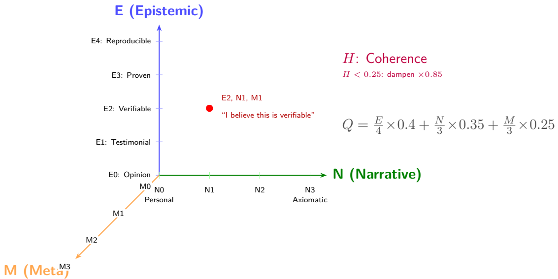
Figure 14.1: The Epistemic Cube: a 3+1 dimensional coordinate system for language generation. The three discrete axes (E, N, M) control assertion strength, social framing, and temporal framing respectively. The holistic axis H (not shown spatially) provides a global coherence dampen. The red dot shows an example coordinate with its natural language implication.
