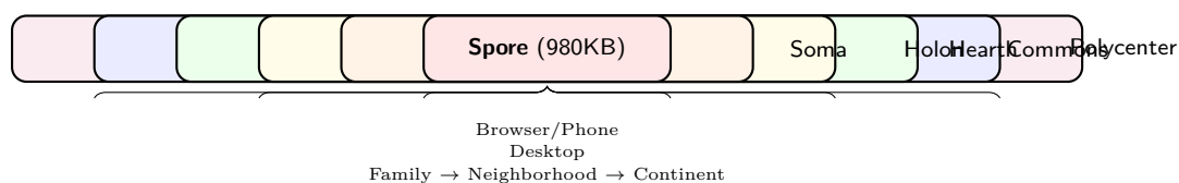
Figure 21.1: Fractal layer nesting: each layer wraps the one below, sharing the same SporeEngine::cycle() API. The innermost Spore kernel (980 KB WASM) runs in browsers; the outermost Polycenter layer coordinates continental governance.
