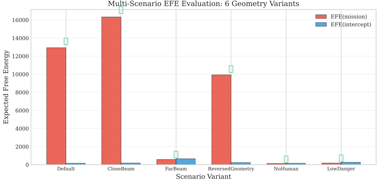
Figure 10: Multi-scenario EFE evaluation. Checkmarks indicate correct decisions. The agent intercepts when safety EFE dominates (Default, CloseBeam, Reversed) and continues the mission otherwise (FarBeam, NoHuman, LowDanger).
