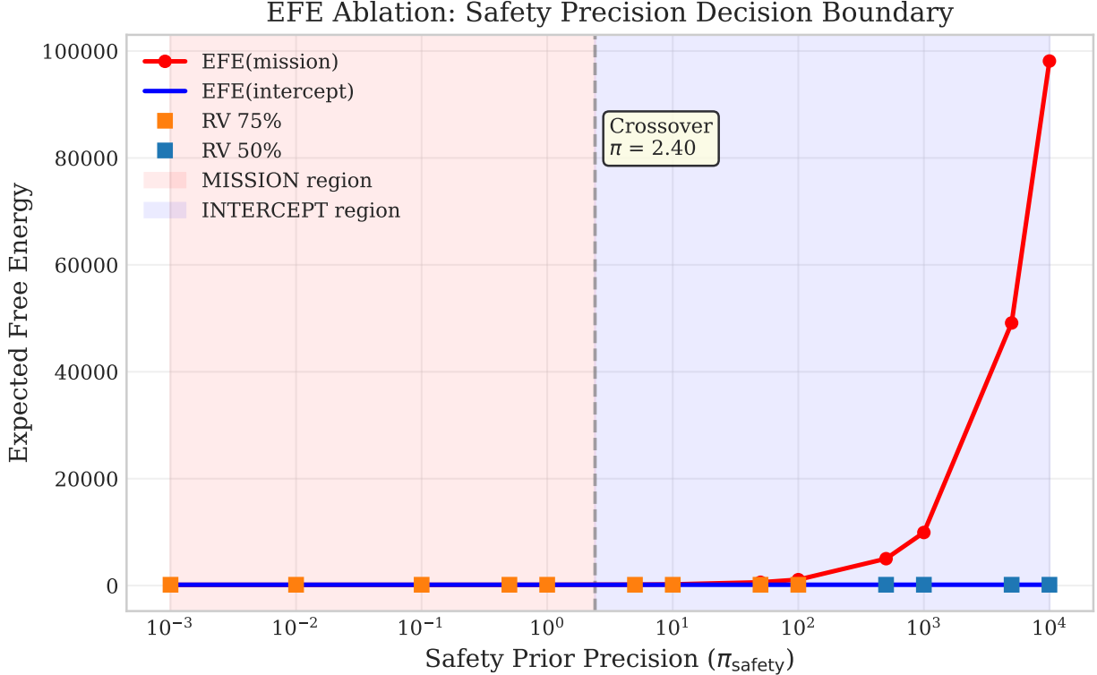
Figure 9: EFE ablation: sweeping safety precision reveals a sharp decision boundary at \pi_{\text{safety}} \approx 2.40 . Below the crossover, mission EFE dominates (red); above, the agent chooses interception (blue). Marker color indicates the winning rendezvous fraction: orange = 75% of impact time (favored at low \pi ), blue = 50% (favored at high \pi ). Note that G(\text{intercept}) plateaus at high precision because successful interception eliminates danger ( \hat{d} \approx 0 ), making \pi_{\text{safety}} \cdot \hat{d}^2 \approx 0 regardless of \pi .
