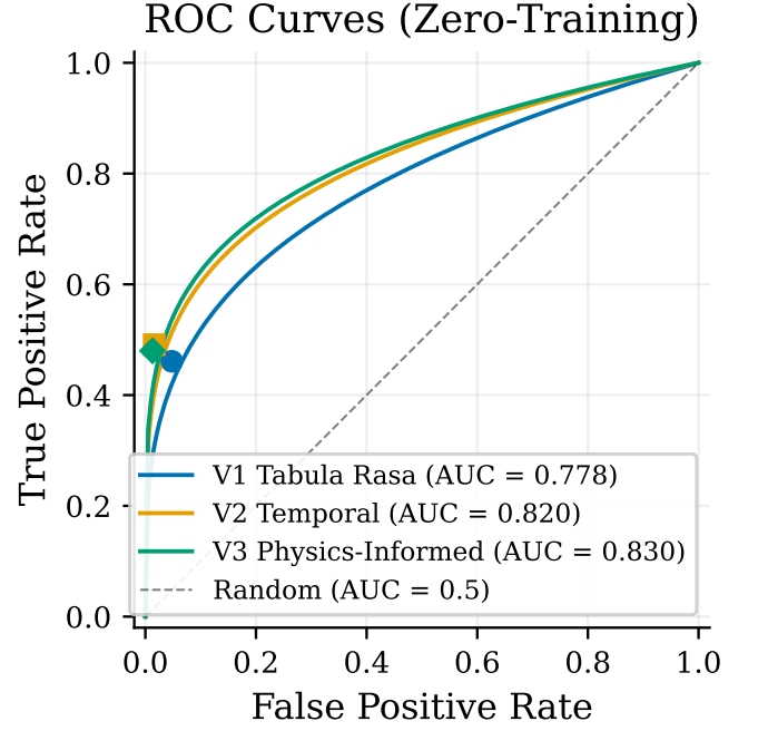
FIG. 3. ROC curves for V1 (Tabula Rasa), V2 (Temporal Self-Reference), and V3 (Physics-Informed) architectures. The diagonal represents random classification (AUC = 0.5). All three curves lie well above the diagonal despite zero gradient-based training.
