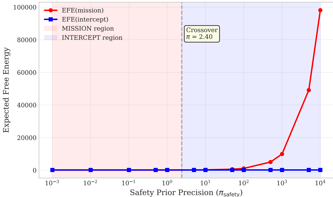
EFE Ablation: Safety Precision Decision Boundary
